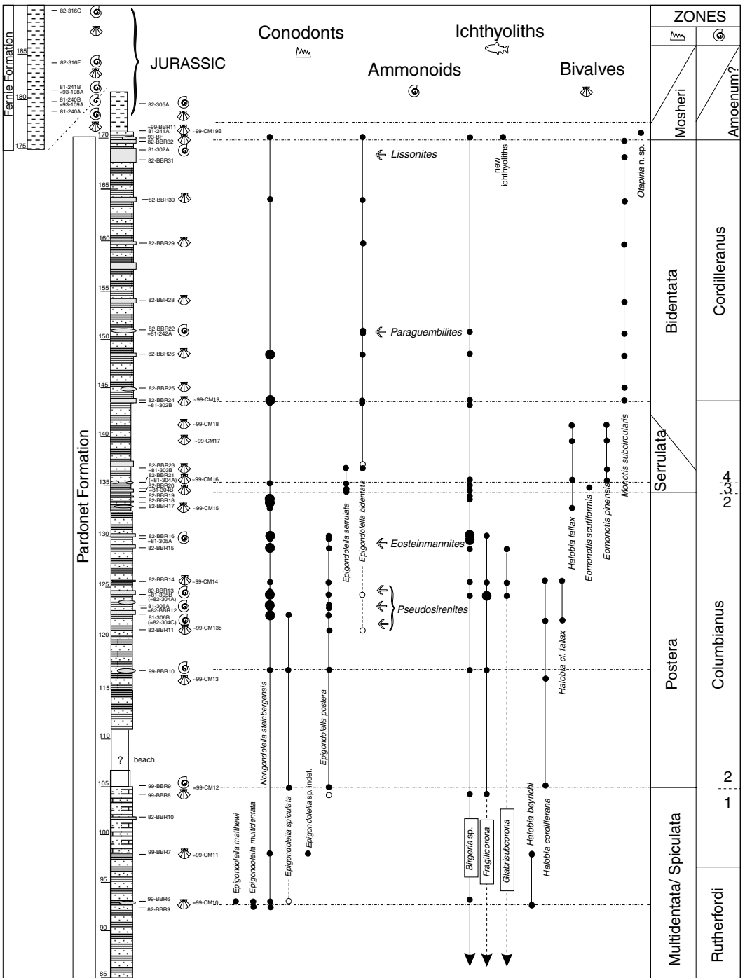
Figure 3. Schematic section of the Middle-Upper Norian and younger part of the Black Bear Ridge section showing occurrence and distribution of conodonts, ammonoids, bivalves, and ichthyoliths within the upper Pardonet and lowest Fernie formations. On the left are shown numbered samples which were taken for conodonts and/or ammonoids, and bivalves (CM). Ichthyolith fauna was recovered from the former. See text for lithological descriptions.
