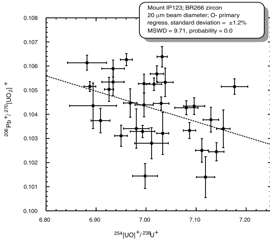
Figure 3. A plot of ^{254}[\text{UO}]^+ / ^{238}\text{U}^+ vs. ^{206}\text{Pb}^+ / ^{270}[\text{UO}_2]^+ for individual SHRIMP analyses of BR266 zircon from mount IP123 (error bars are 1\sigma ). An O- primary beam was used to analyze spots approximately 20 \mu\text{m} wide by 1 \mu\text{m} deep. No correction for common Pb was made, but it is insignificant for these data. A linear least-squares fit to the dependent variable ^{206}\text{Pb}^+ / ^{270}[\text{UO}_2]^+ is shown, generating a calibration curve assumed to correspond with the TIMS ^{206}\text{Pb} / ^{238}\text{U} age of the zircon.
