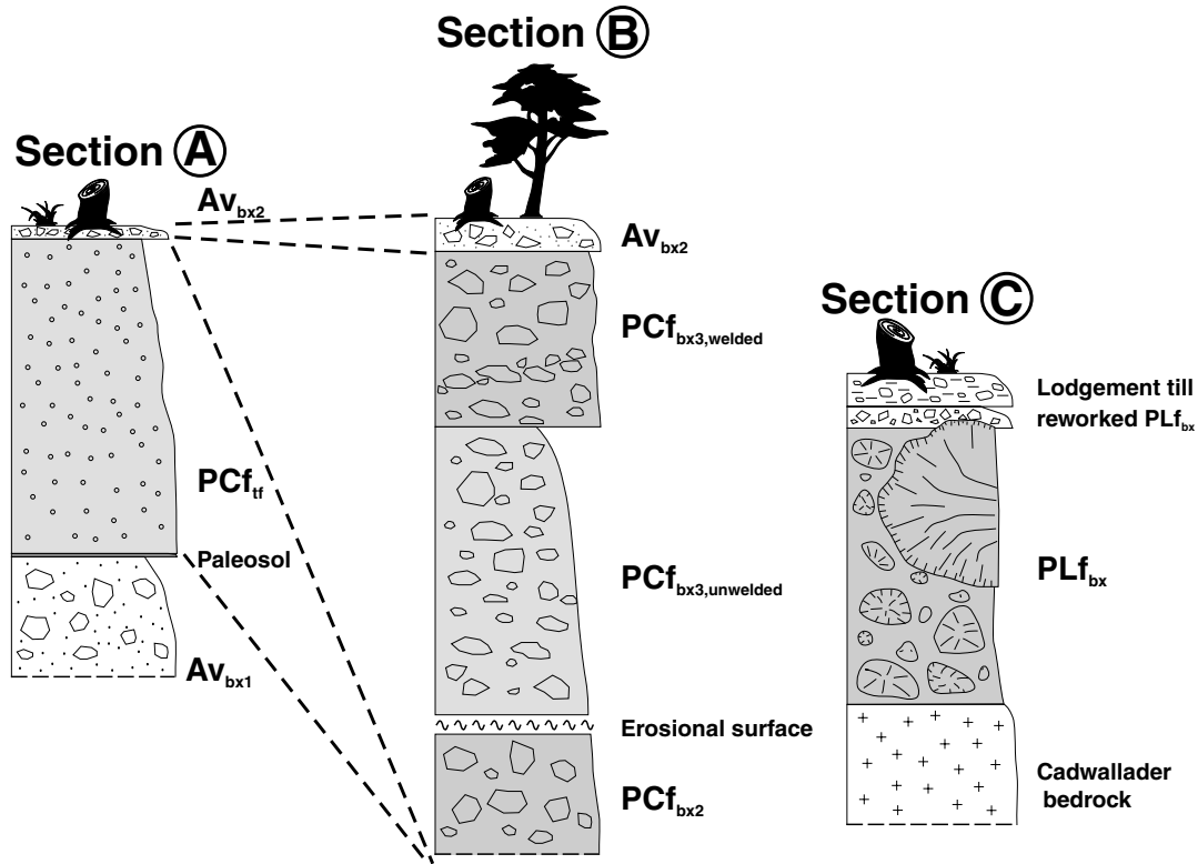
Figure 3. Schematic stratigraphic sections summarizing the distribution and stratigraphic relationships of major units of the Pebble Creek Formation. Locations are keyed to the geological map (Fig. 2) by letters: A) western limit of the Plinth avalanche overlying pyroclastic fall, B) eastern toe of the Plinth avalanche overlying late Pebble Creek block-and-ash flows, C) Plinth block-and-ash outlier sitting on bedrock upslope and east of B). Unit names and codes are the same as in Figure 2 (see text). Shaded units are volcanic in origin.
