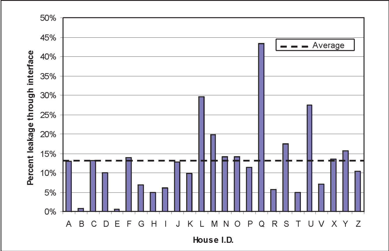
Figure 1: Percent of House Air Leakage Through House/Garage Interface
