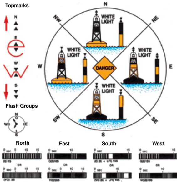
Figure 11-4 Cardinal Buoys
