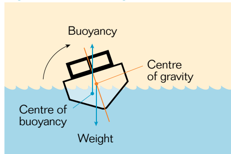
Figure 8-2 Heeling
