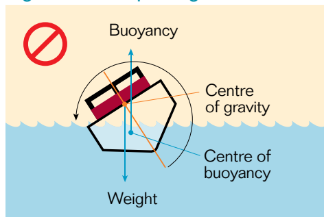
Figure 8-4 Capsizing
