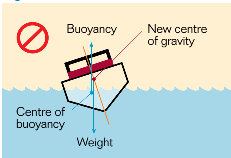
Figure 8-3 Added Load
