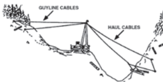
Figure 2.1 – Highlead Spar
