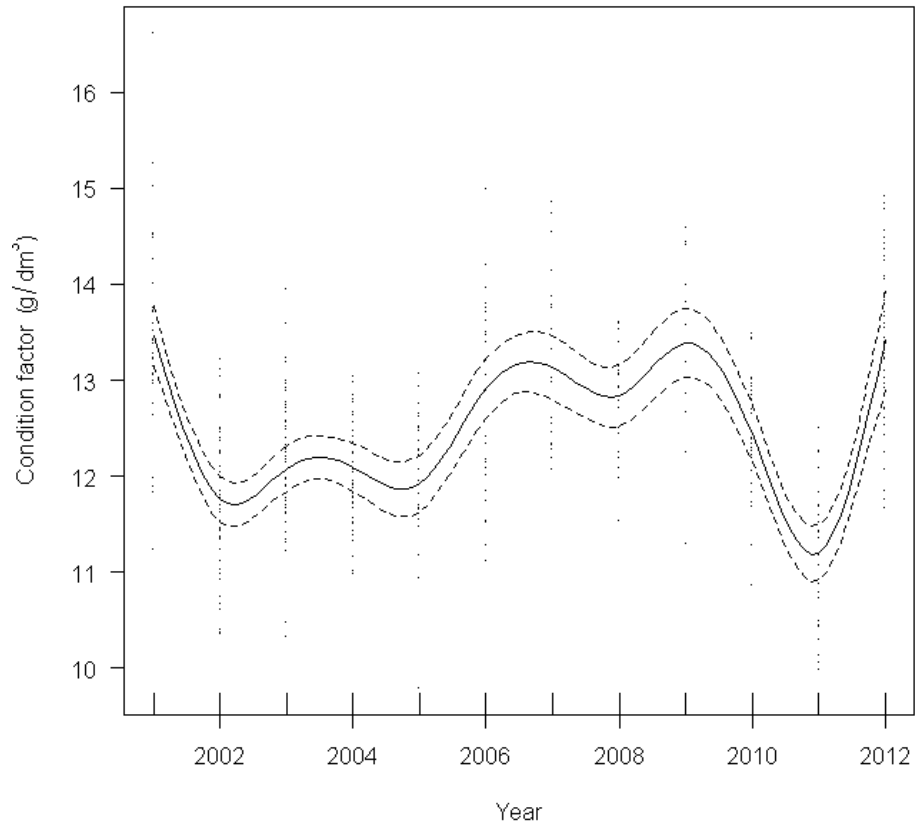
Figure 17. Fit of condition factor (g/dm 3 ) as a function of year from a generalized additive model. Shows the annual trend in condition factor for scallops from the annual surveys of SFA 29 West (2001–2012).
