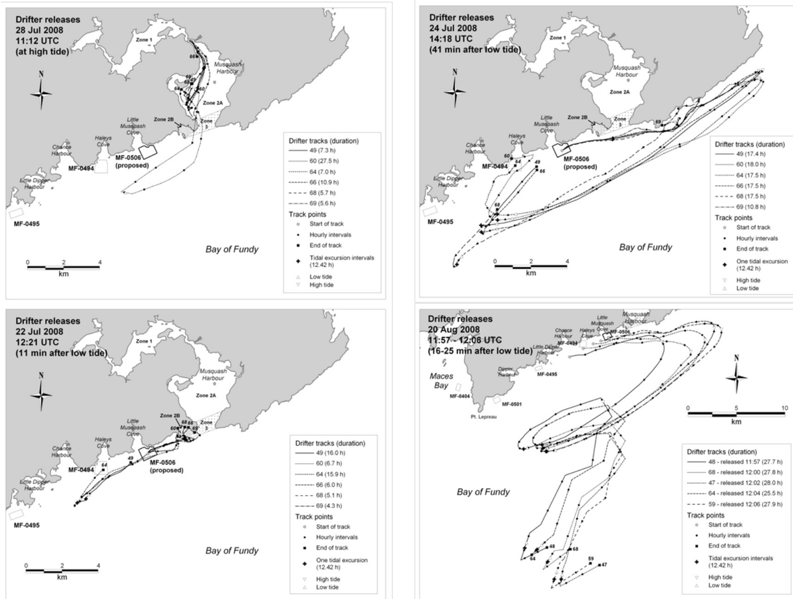
Figure 12. Sample drifter tracks from the Musquash area (from Page et al. 2009).
