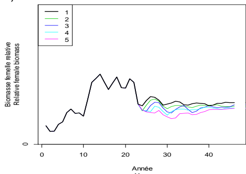
C) Relation stock-recrutement de type Ricker
