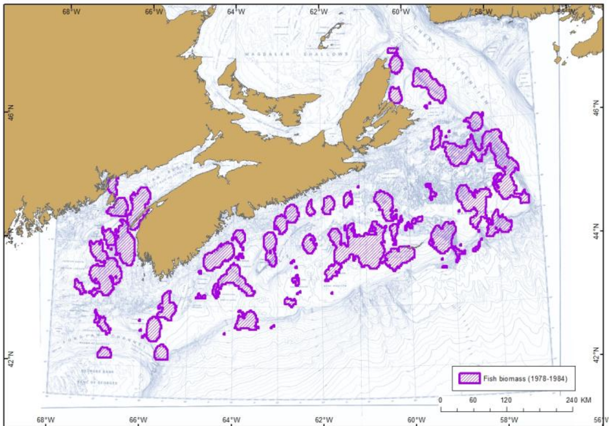
Figure 3. Areas of high fish biomass for the period of 1978 to 1984 based on the DFO summer Research Vessel data.
