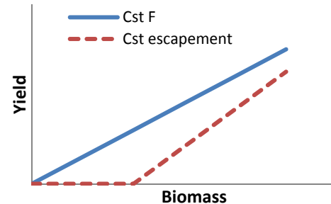
Figure 2. Illustration of control rules featuring constant fishing rate alone or coupled with a limit biomass (constant escapement).
