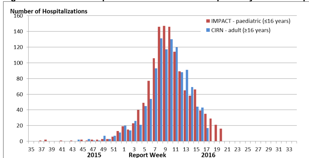
2015-16, pediatric and adult hospitalizations ( \leq 16 years of age, IMPACT; \geq 16 years of age, CIRN-SOS)*
