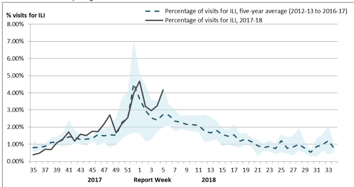
Figure 4 – Percentage of visits for ILI reported by sentinels by report week, Canada, weeks 2017-35 to 2018-05
