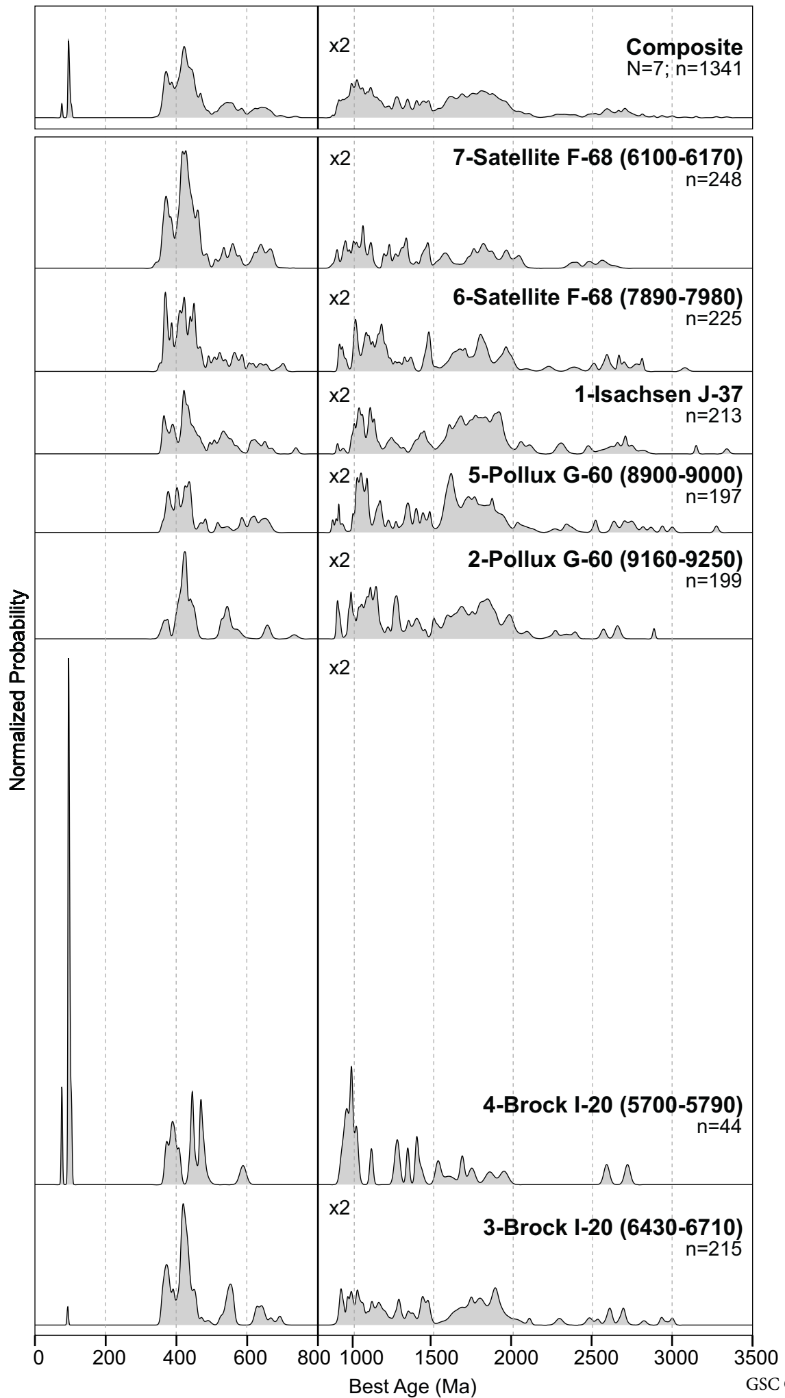
Figure 5 - Normalized Detrital Zircon Probability Density Plots
