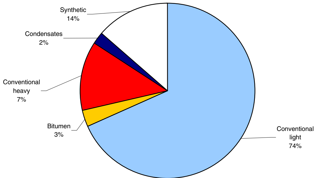
Refinery supply of crude oils - by type - June 2005
