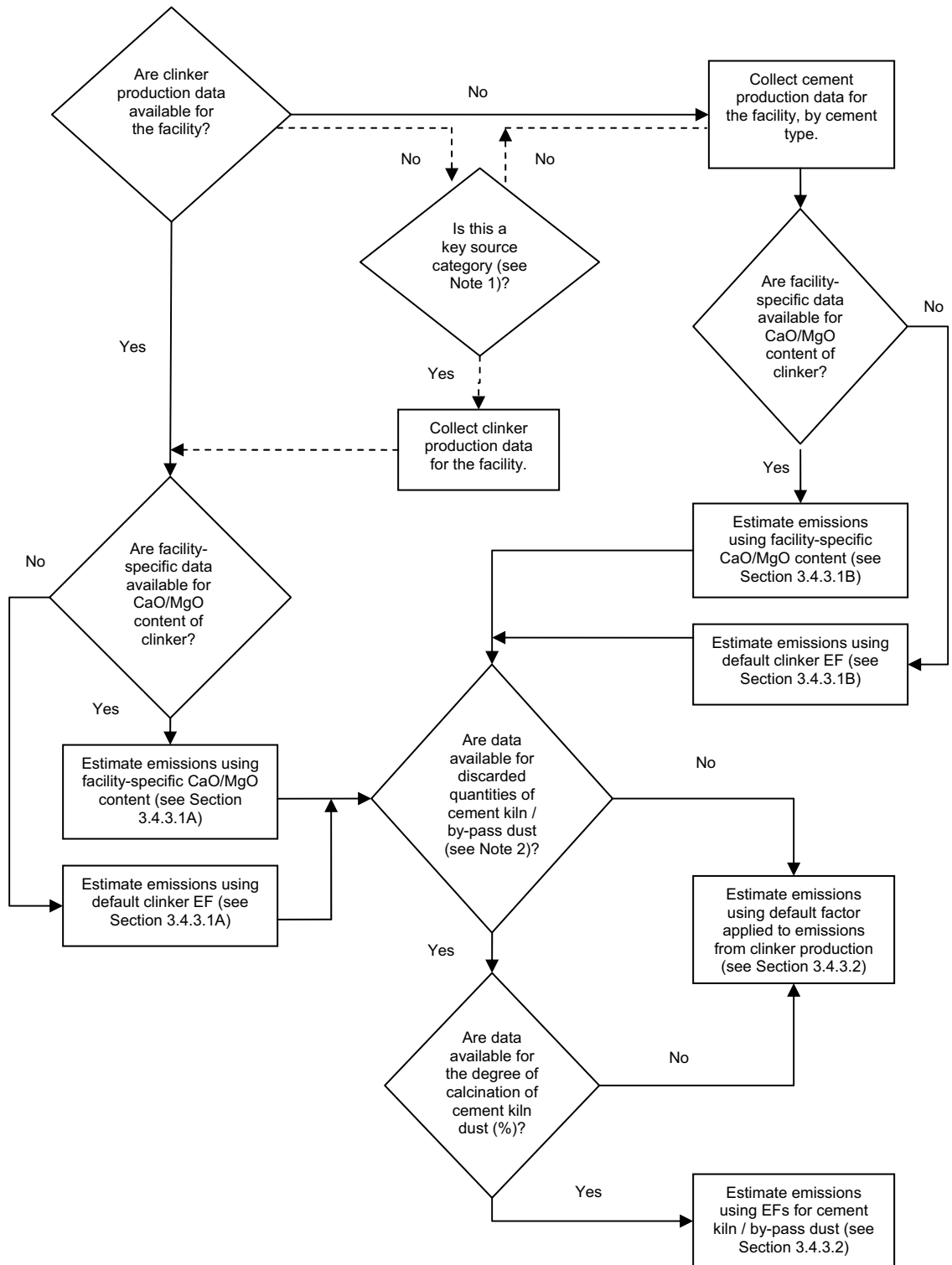
Figure 3: Decision Tree for Selecting the Method for Estimating CO 2 Emissions from Clinker Production
