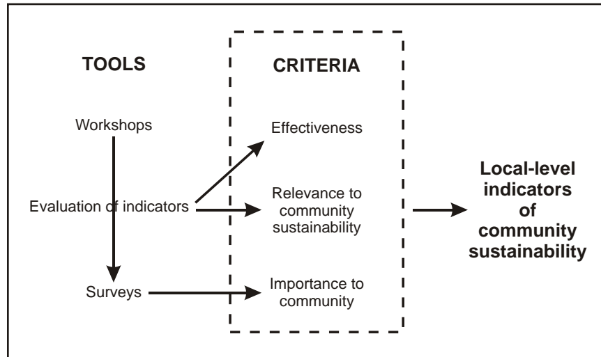
Figure 2. Selection process for local-level indicators.
