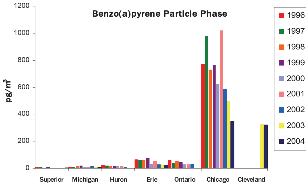
Figure 8A-7. Annual Average Particle-phase B(a)P Concentrations (pg/m 3 ) 37
