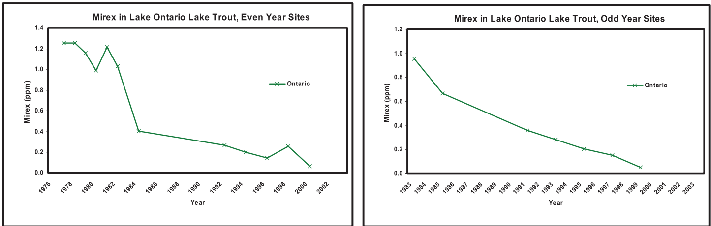
Figure 8F-8. Mirex in Lake Ontario Lake Trout, Even Year (left) and Odd Year (right) Sites. Source: US EPA GLNPO Great Lakes Fish Monitoring Program
