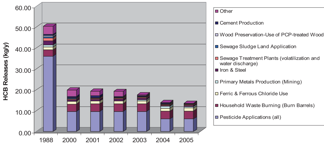
Figure 4-1. Estimated HCB Releases (to air and water) in Ontario by Sector, 1988-2005. Source: Environment Canada (Environmental Protection Operations Division – Ontario Region) Inventory as of Nov. 2006, with an update on releases from pesticide application received from Health Canada’s Pest Management Regulatory Agency (Letter dated April 11, 2005)
