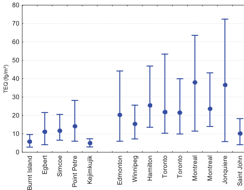
Figure 3-6. 2,3,7,8-TCDD TEQ Concentrations (fg/m³) 2003-2005 (Mean, 10th and 90th percentiles). Source: Environment Canada 14
