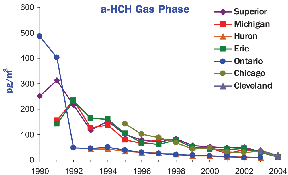
Figure 8A-4. Annual Average Gas-phase Concentrations of Alpha-HCH (pg/m³) 34
