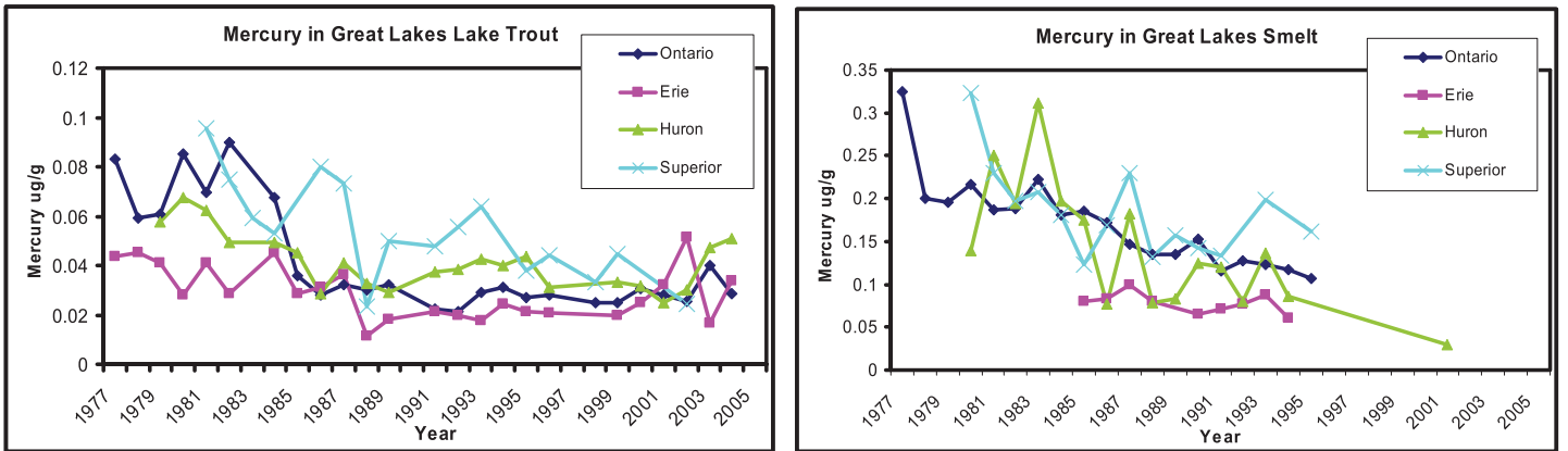
Figure 8F-5. Mercury in Great Lakes Lake Trout (left) and Great Lakes Smelt (right). Source: Environment Canada Great Lakes Fish Surveillance Program
