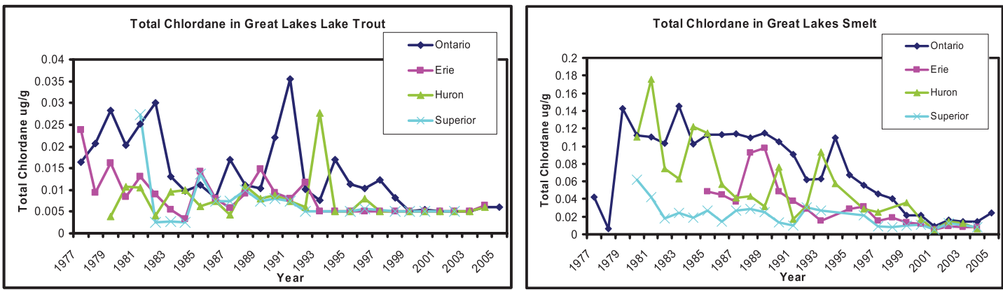
Figure 8F-7. Total Chlordane in Great Lakes Lake Trout (left) and Great Lakes Smelt (right). Source: Environment Canada Great Lakes Fish Surveillance Program
