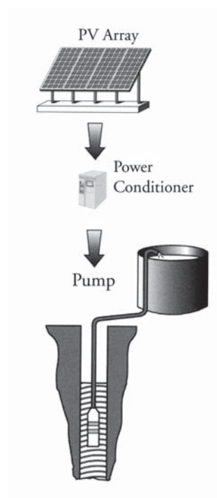
Figure 7: Water Pumping PV System Schematic [adapted from Ross and Royer, 1999].
