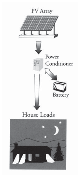
Figure 5: Stand-Alone Off-Grid PV System Schematic [adapted from Ross and Royer, 1999].
