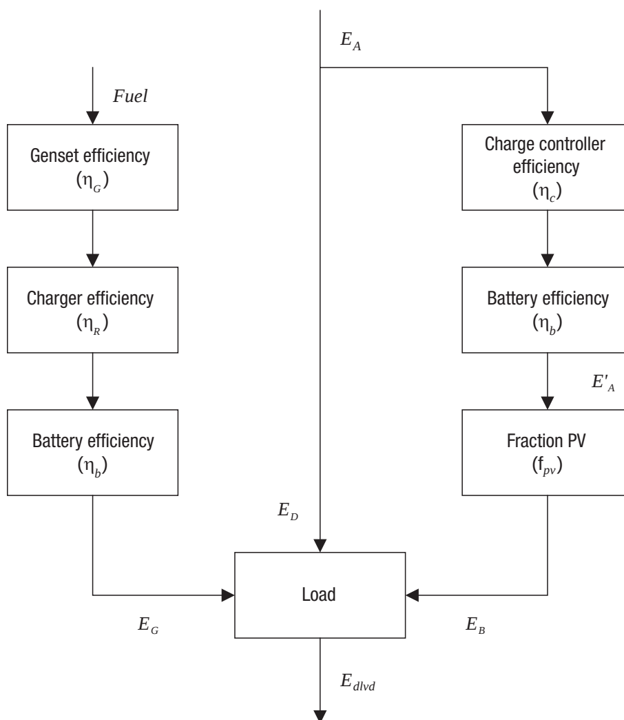
Figure 12: Flowchart for PV Off-Grid Model.
