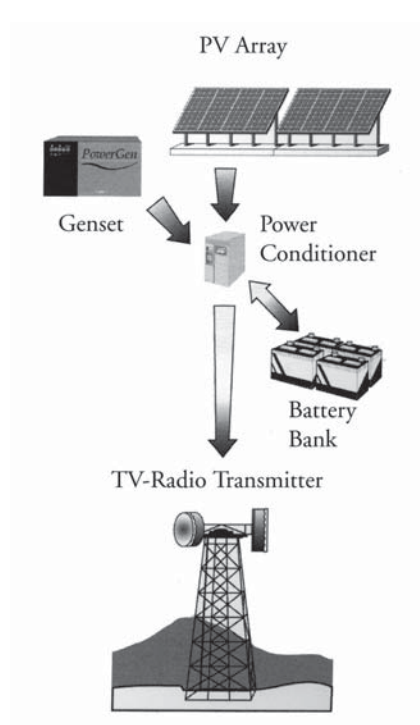
Figure 6: Hybrid Off-Grid PV System Schematic [adapted from Ross and Royer, 1999].
