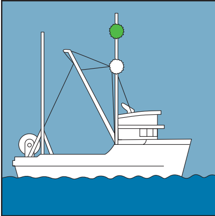
STARBOARD VIEW
