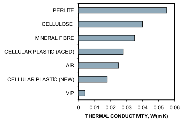
Thermal conductivity of VIP compared to several common insulating materials. (Please note that the graph represents current, practical lower limits of thermal conductivity for the generic insulation materials.)
