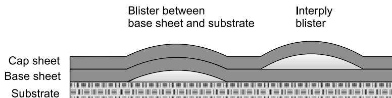
Figure 1. Blistering locations in modified bituminous membranes
