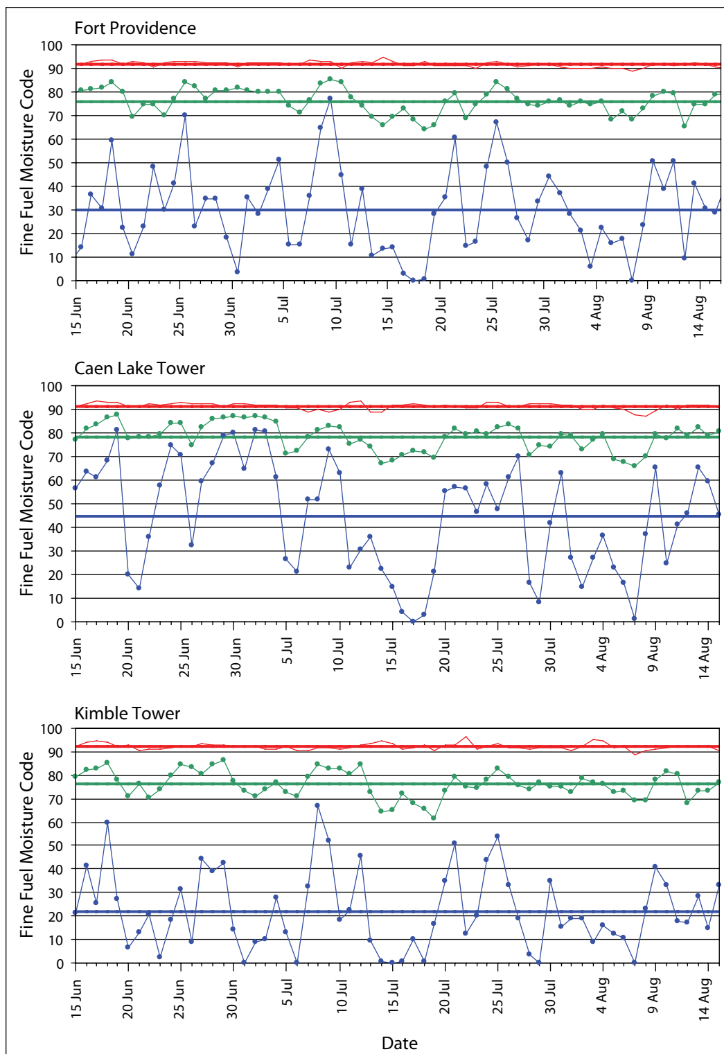
Figure 17. Minimum (blue), maximum (red), and average (green) standard daily Fine Fuel Moisture Code for each day of the peak fire season and associated total averages for the period (see Table 1 for years of data available for each weather station).
