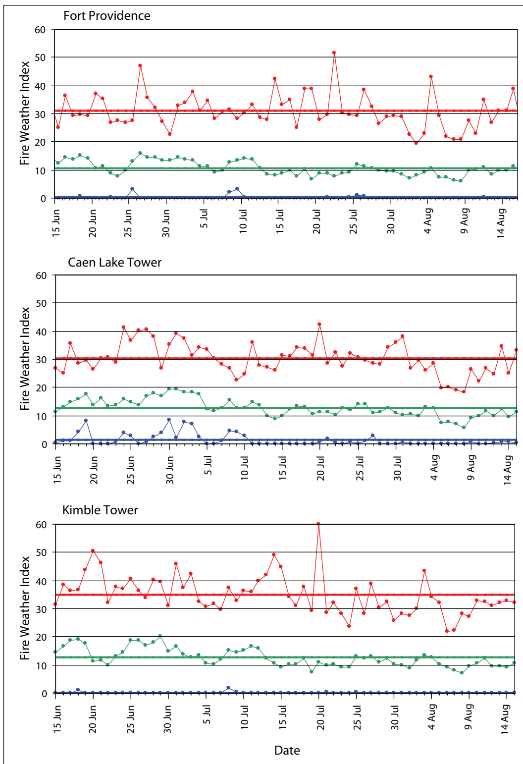
Figure 27. Minimum (blue), maximum (red), and average (green) standard daily Fire Weather Index for each day of the peak fire season and associated total averages for the period (see Table 1 for years of data available for each weather station).
