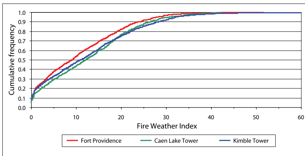
Figure 28. Cumulative frequency of the standard daily Fire Weather Index for the three weather stations.
