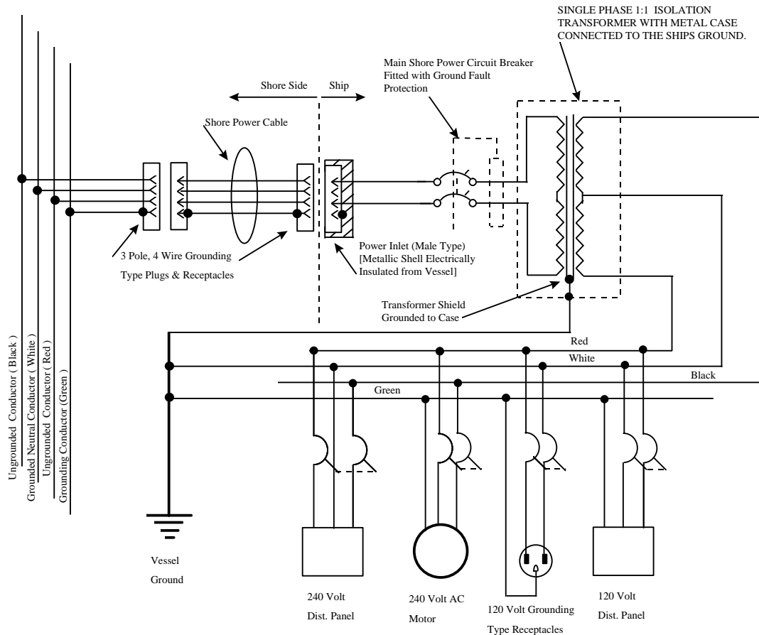
FIGURE 11-2 ISOLATION TRANSFORMER SYSTEM WITH SINGLE PHASE 240 VOLT INPUT AND 120/24- VOLTAGE PHASE OUTPUT WITH GF PROTECTION OF TRANSFORMER PRIMARY
