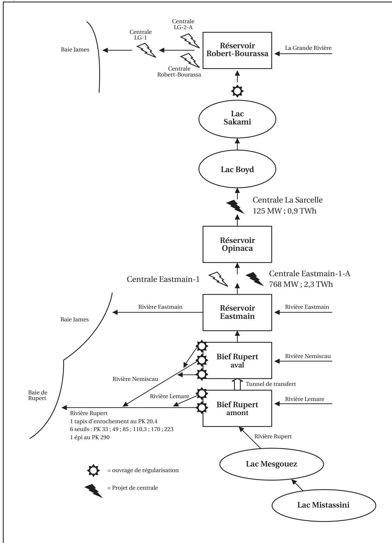
Figure 2-2 Schematic diagram of the Eastmain-1-A and Rupert diversion project
