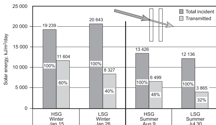
Figure 3. Measured transmitted solar energy on sunny days from the CCHT experiment
