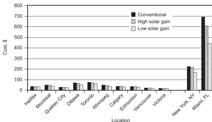
Figure 5. Annual cost of cooling for North American locations (costs are represented in each country's currency)
