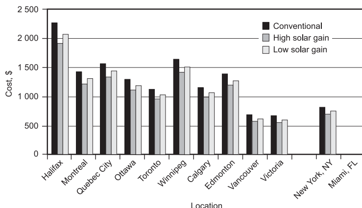
Figure 4. Annual cost of heating for North American locations (costs are represented in each country's currency)
