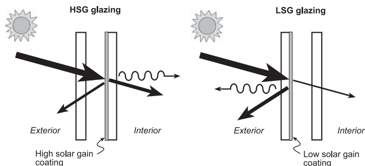
Figure 1. High solar heat gain (HSG) and low solar heat gain (LSG) glazing
