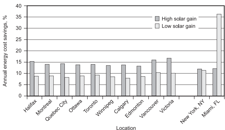
Figure 6. Annual energy cost savings compared to conventional clear glass glazing
