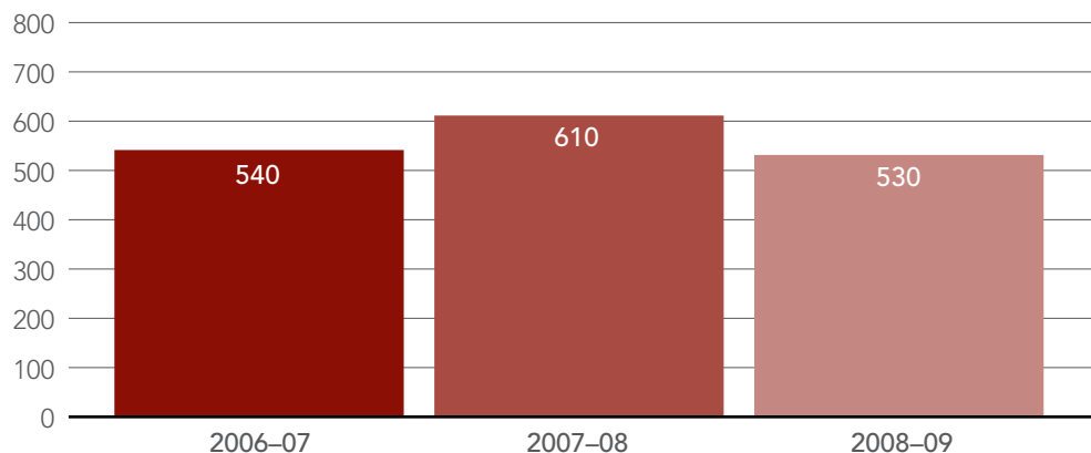
FIGURE 1 TARGETING STATISTICS*
