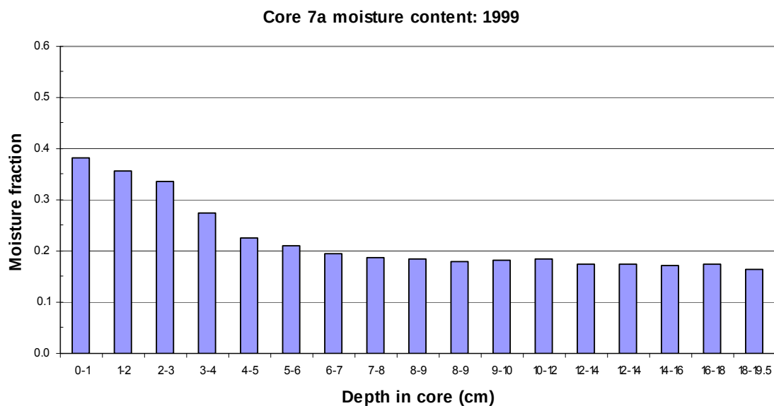
Figure 20. Viscount Melville Sound sediment: moisture fraction vs depth in core.
