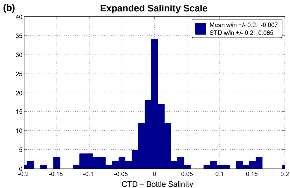
Figure 12. Histograms showing CTD-Bottle salinity differences with a -1 m offset applied in (a) full scale and (b) expanded salinity scale.
