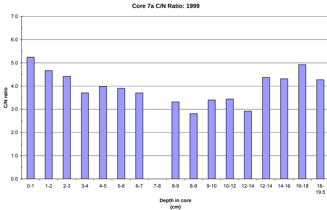
Figure 16. Viscount Melville Sound sediment: C/N ratio vs depth in core.
