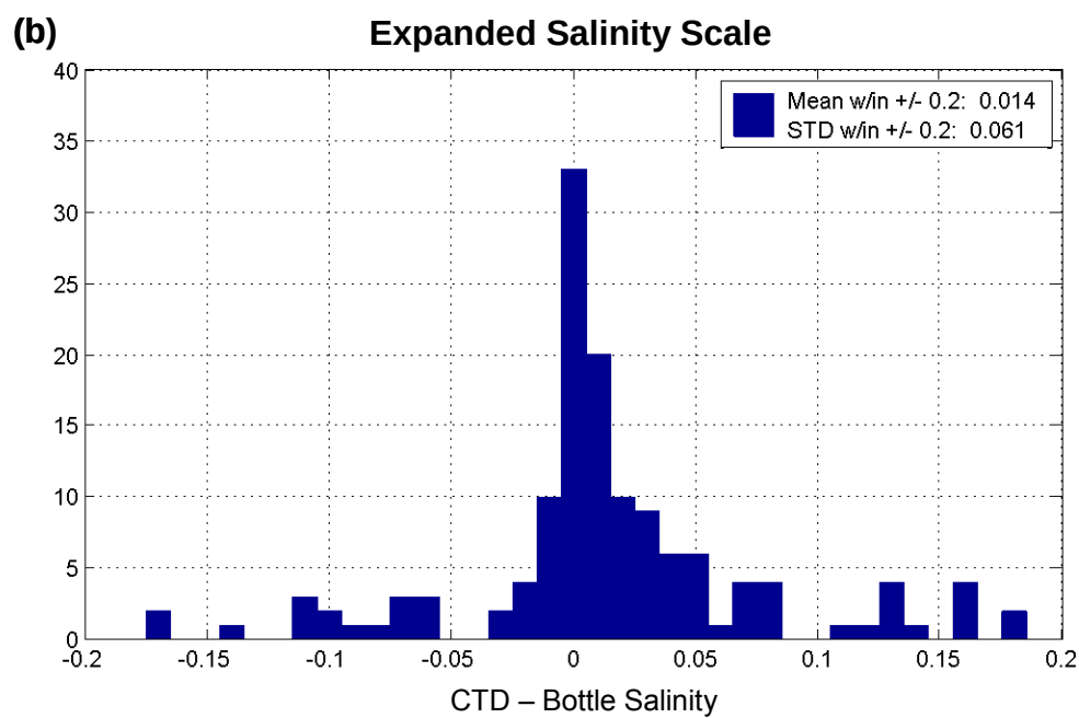
Figure 10. Histograms showing CTD-Bottle salinity differences with a +1 m offset applied in (a) full scale and (b) expanded salinity scale.
