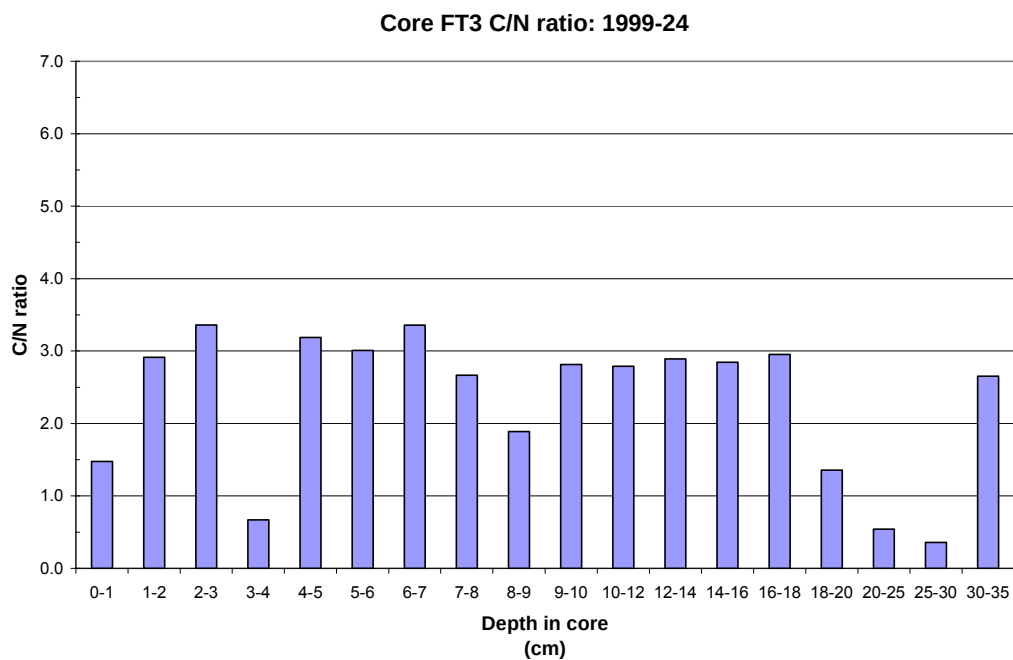
Figure 19. Peel Sound sediment: C/N ratio vs depth in core.
