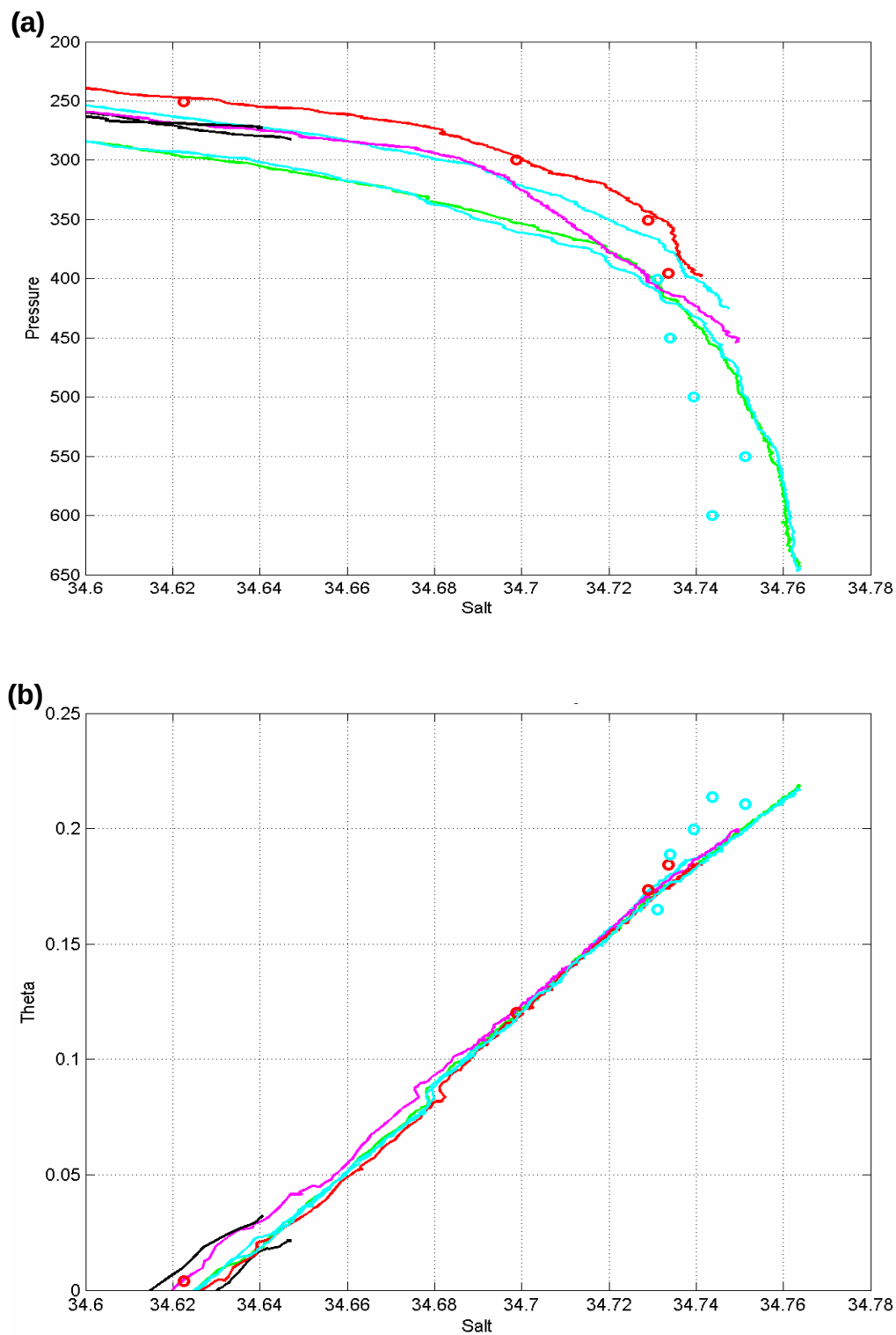
Figure 13. (a) Salinity profile and (b) Theta - Salinity plot. These figures show larger CTD v. Bottle differences in the deep waters of Amundsen Gulf.
