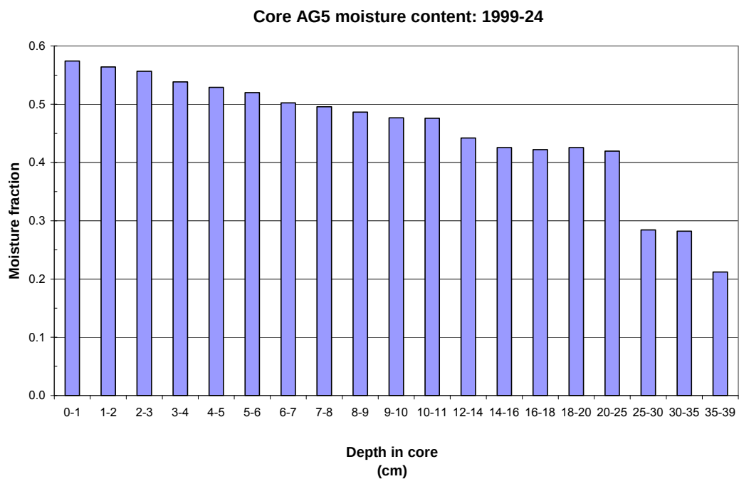
Figure 22. Amundsen Gulf sediment: moisture fraction vs depth in core.
