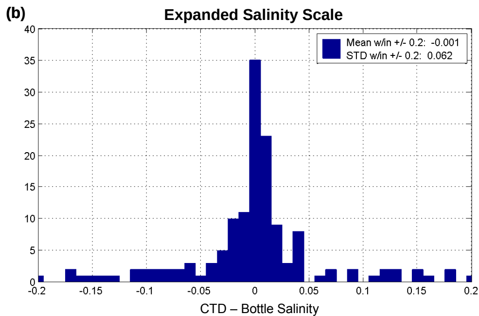
Figure 11. Histograms showing CTD-Bottle salinity differences with a 0 m offset applied in (a) full scale and (b) expanded salinity scale.
