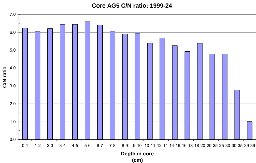
Figure 18. Amundsen Gulf sediment: C/N ratio vs depth in core.
