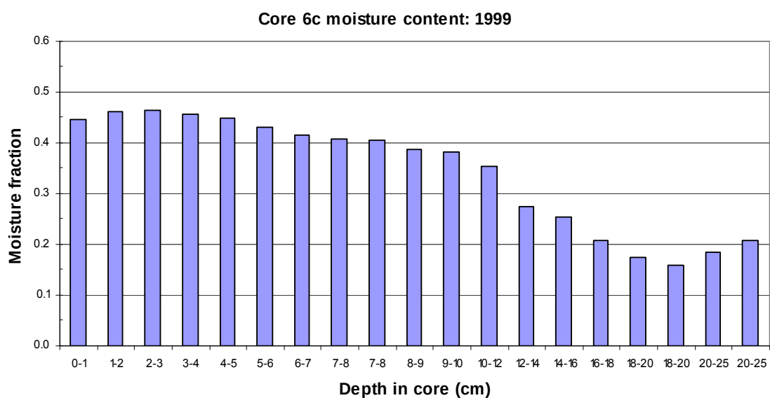
Figure 21. Viscount Melville Sound sediment: moisture fraction vs depth in core.
