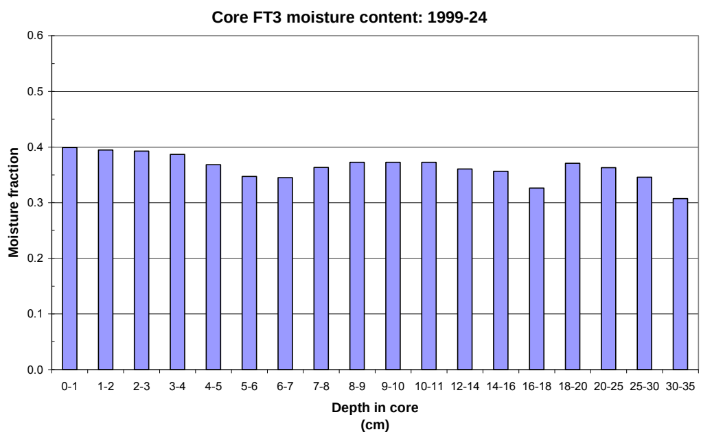
Figure 23. Peel Sound sediment: moisture fraction vs depth in core.
