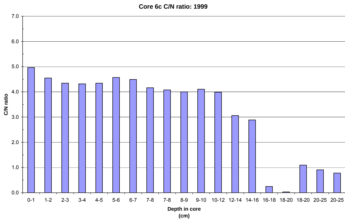
Figure 17. Viscount Melville Sound sediment: C/N ratio vs depth in core.
