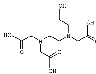
HEDTA (hydroxyethylethylenediaminetriacetic acid)
