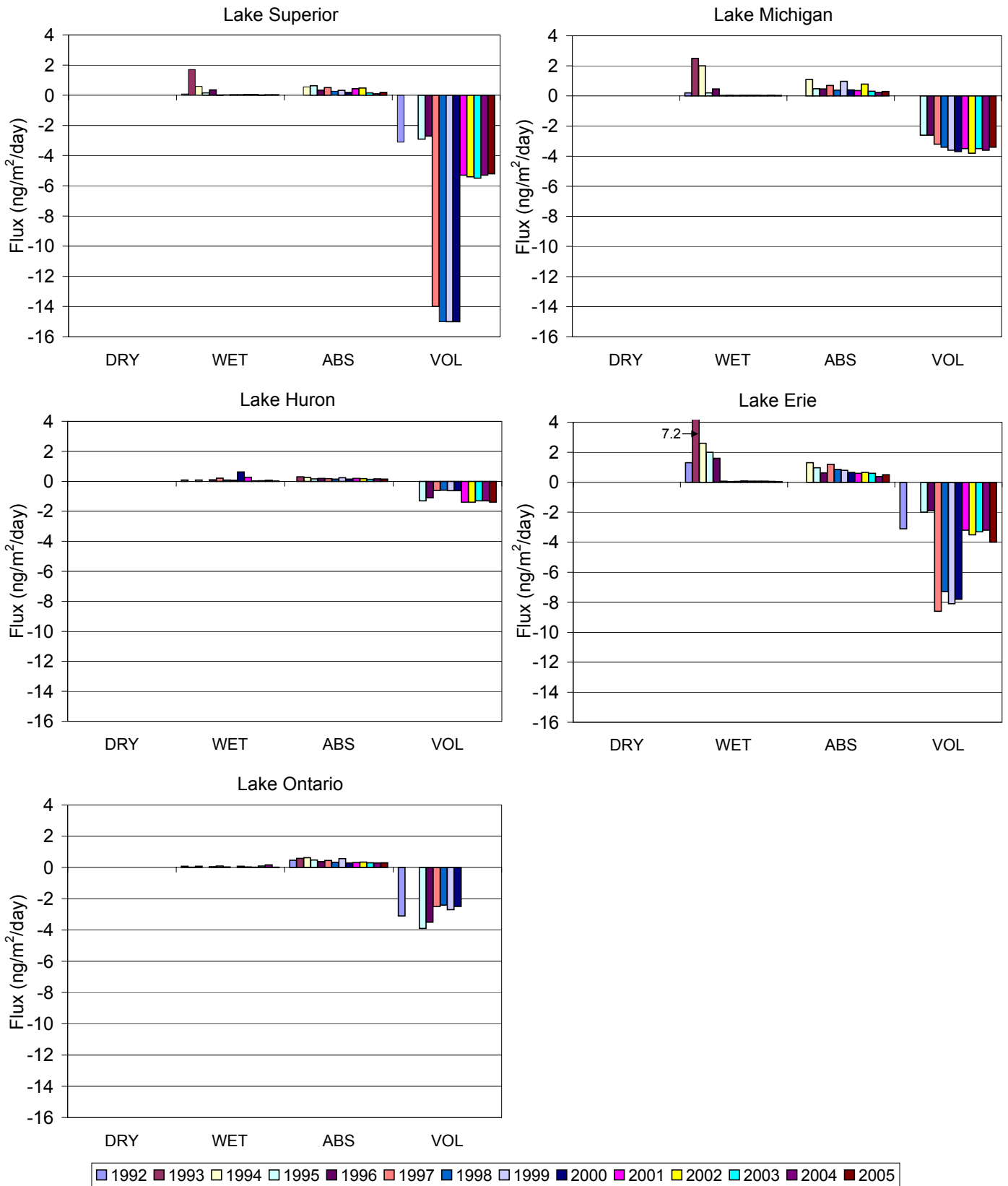
Figure C6: Annual Average Flux (ng/m 2 /day) of trans -chlordane.
