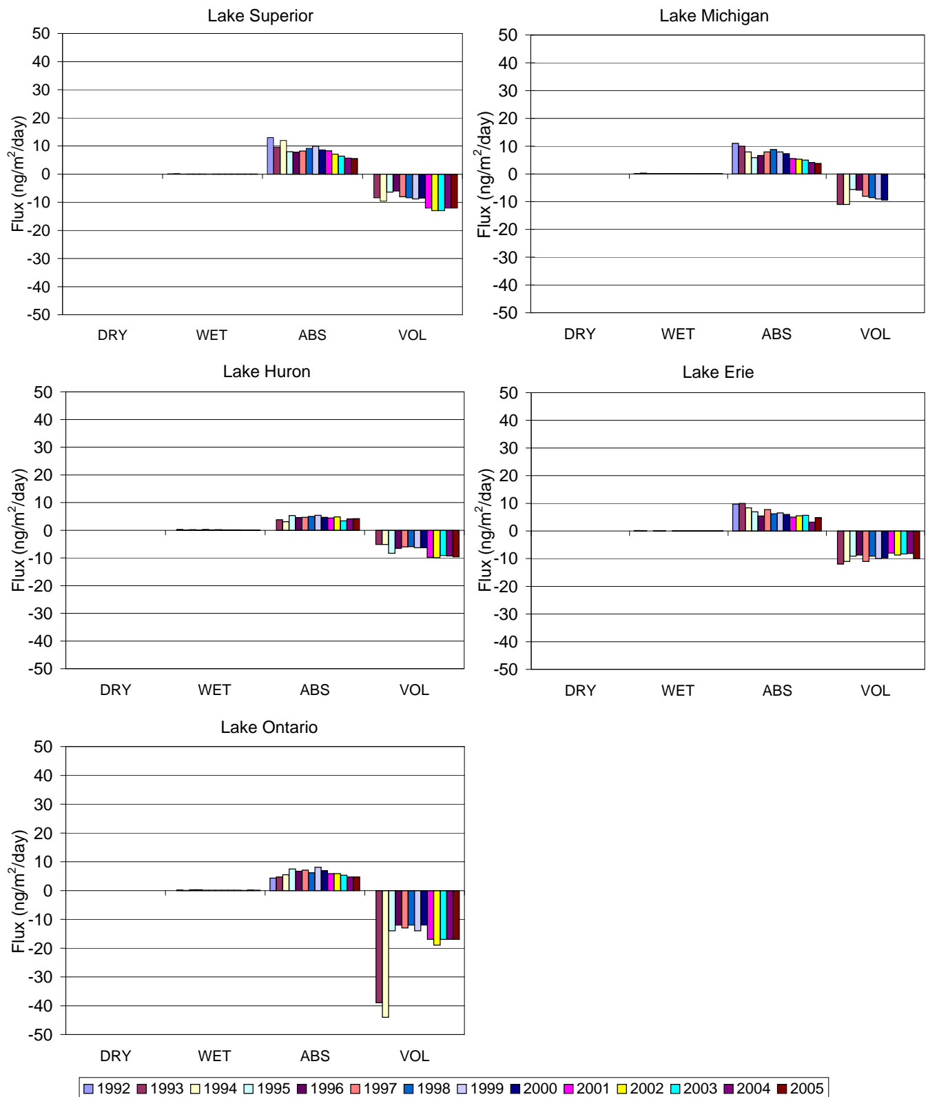
Figure C4: Annual Average Flux ( \text{ng/m}^2/\text{day} ) of hexachlorobenzene.
