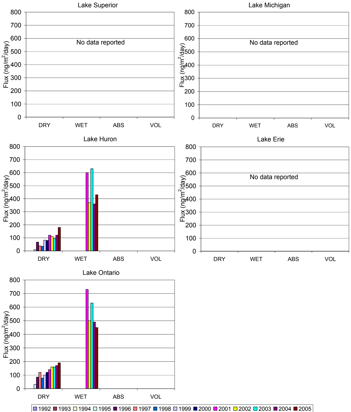
Figure C24: Annual average flux (ng/m 2 /day) of selenium.
