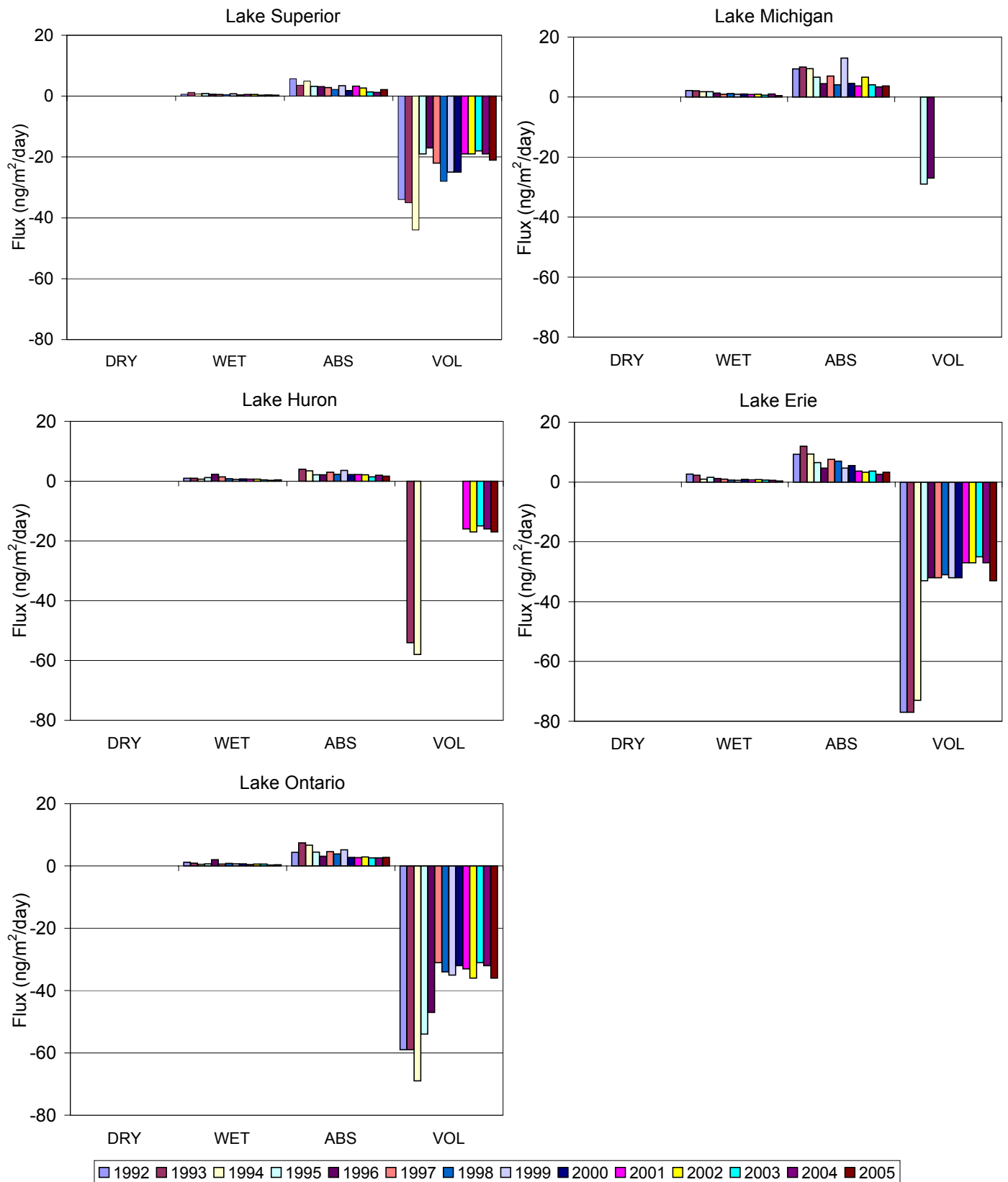
Figure C3: Annual Average Flux ( \text{ng/m}^2/\text{day} ) of dieldrin.
