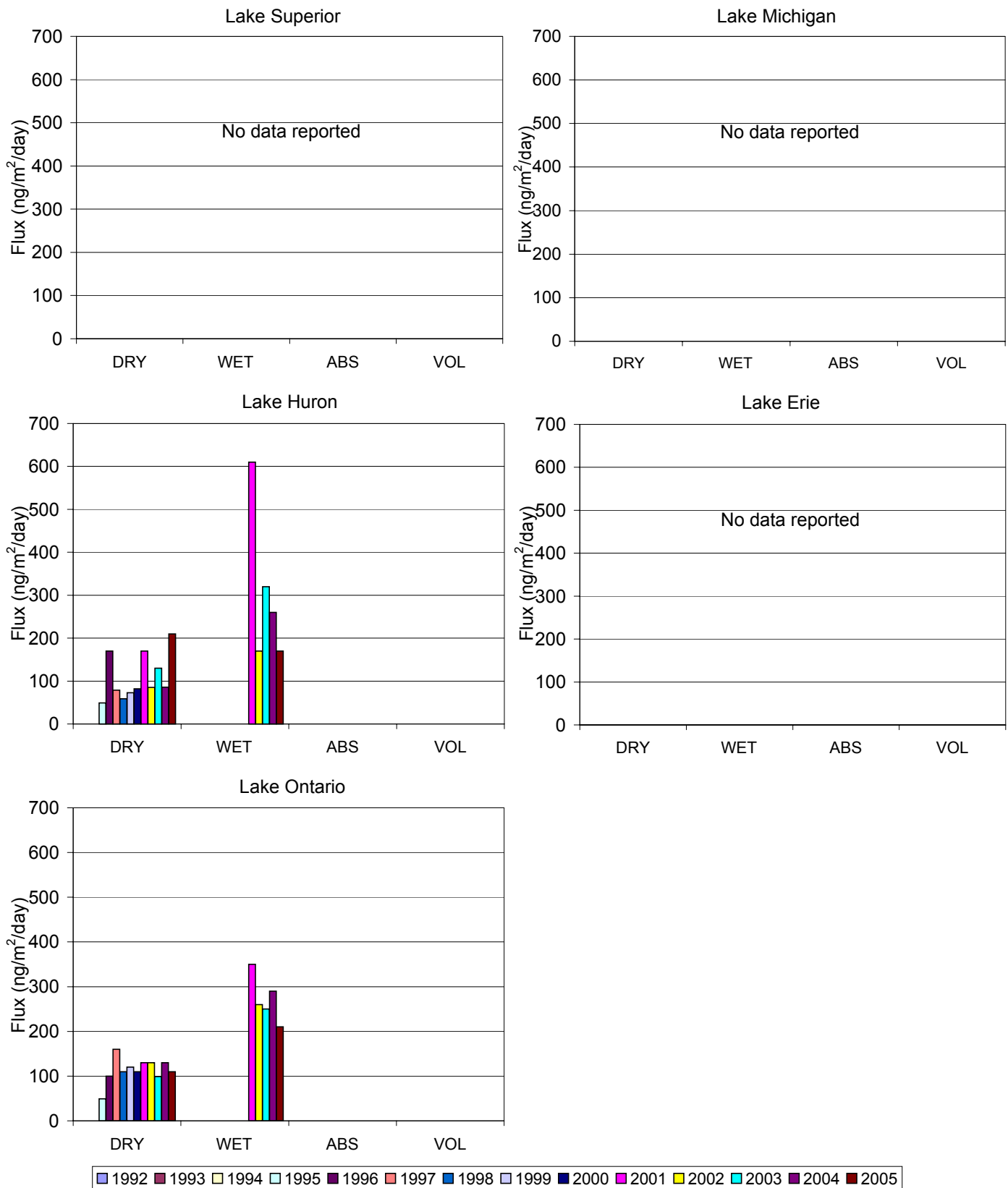
Figure C21: Annual average flux (ng/m 2 /day) of arsenic.
