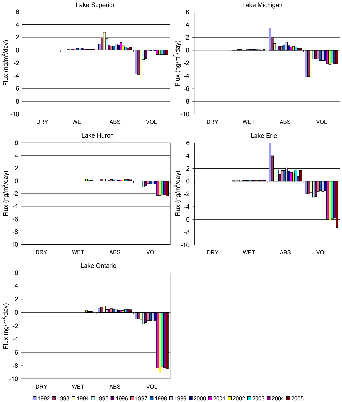
Figure C14: Annual average flux ( \text{ng/m}^2/\text{day} ) of PCB101.
