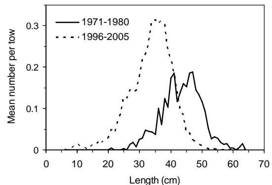
Figure 9. Length composition of catches in the September RV survey of the southern Gulf of St. Lawrence in two periods.
