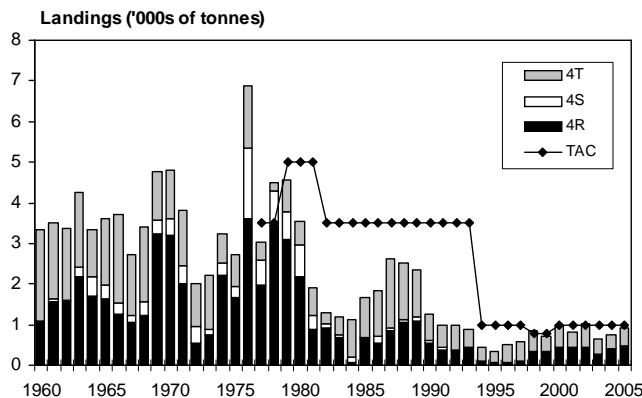
Figure 2. Landings and TAC of 4RST witch flounder.
