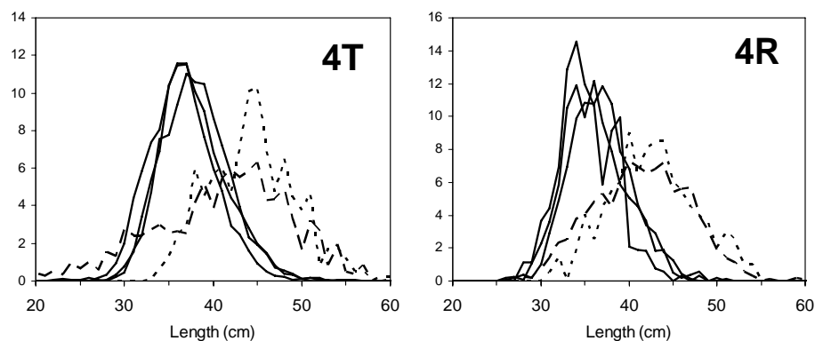
Figure 4. Length distribution (%) of witch flounder landings in recent years (2001, 2003, 2005; solid lines) compared to those in the mid 1970s (dotted line) and early 1980s (dashed line).
