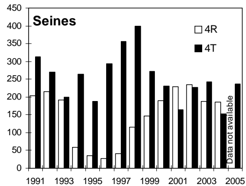
Figure 3. Fishing effort (days) by seines directing for witch flounder.
