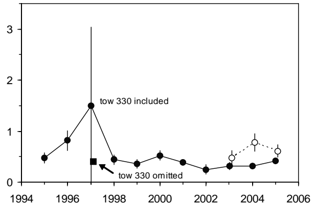
Figure 12. Mean catch rates (kg/tow) in the July sentinel survey of the northern Gulf (closed circles) and the August sentinel survey of the southern Gulf (open circles). Vertical lines are \pm 1 standard error.
