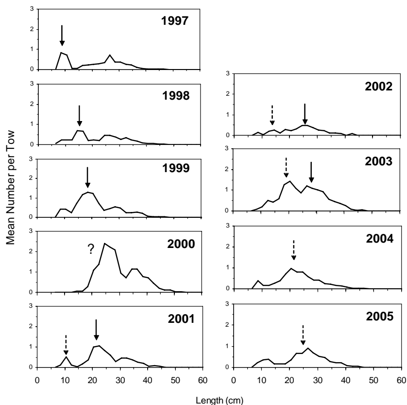
Figure 10. Length composition of catches in the August RV survey of the northern Gulf of St. Lawrence. Arrows mark the progression of year-classes through the length frequencies.
