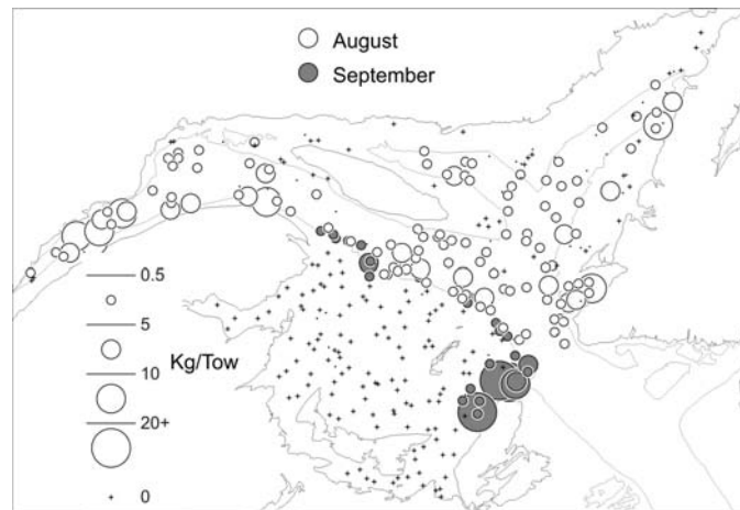
Figure 7. Geographic distribution of witch flounder in the summer RV surveys of the Gulf of St. Lawrence.
