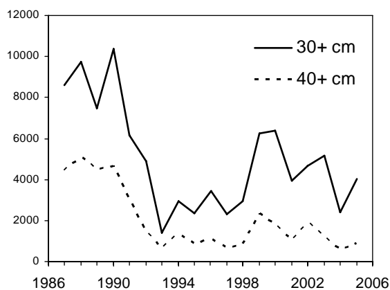
Figure 5. Biomass index for commercial sizes of witch flounder.
