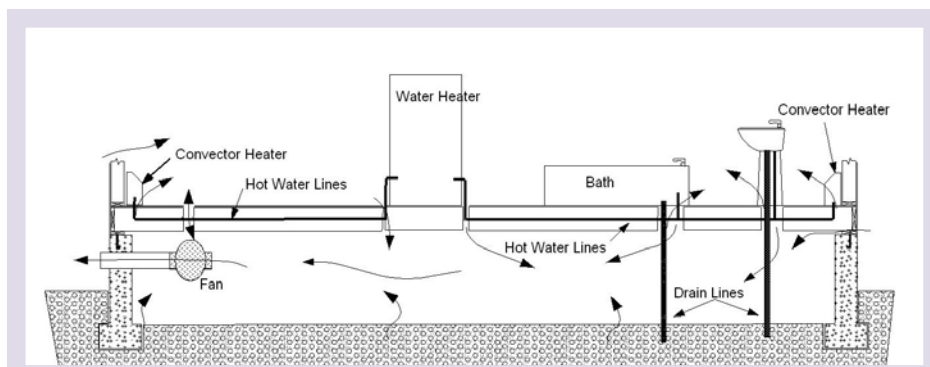
Figure 14 – Crawlspace Exhaust
