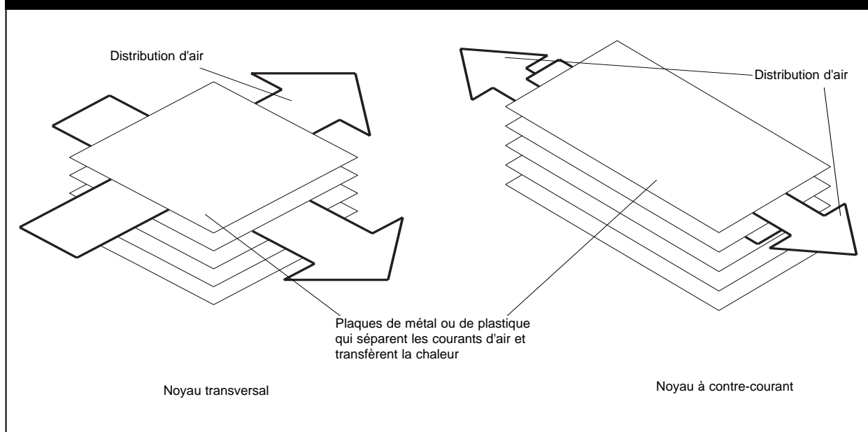
Figure 40 : HRV à plaque
