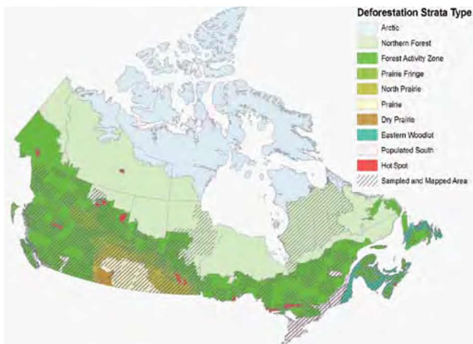
Figure A3–9 Forest Conversion Strata and Areas Sampled for the 2012 Submission
