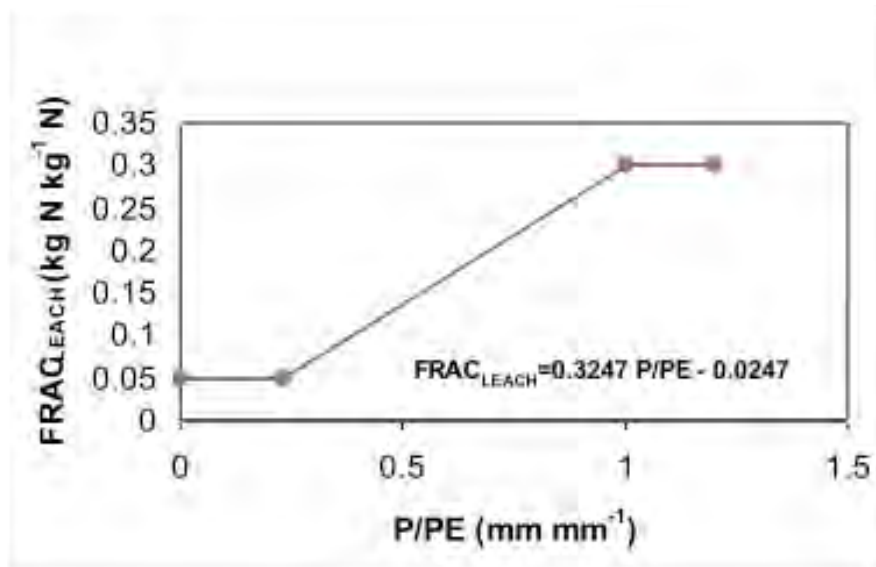
Figure A3-4 Determination of the Ecodistrict FRAC LEACH Values
