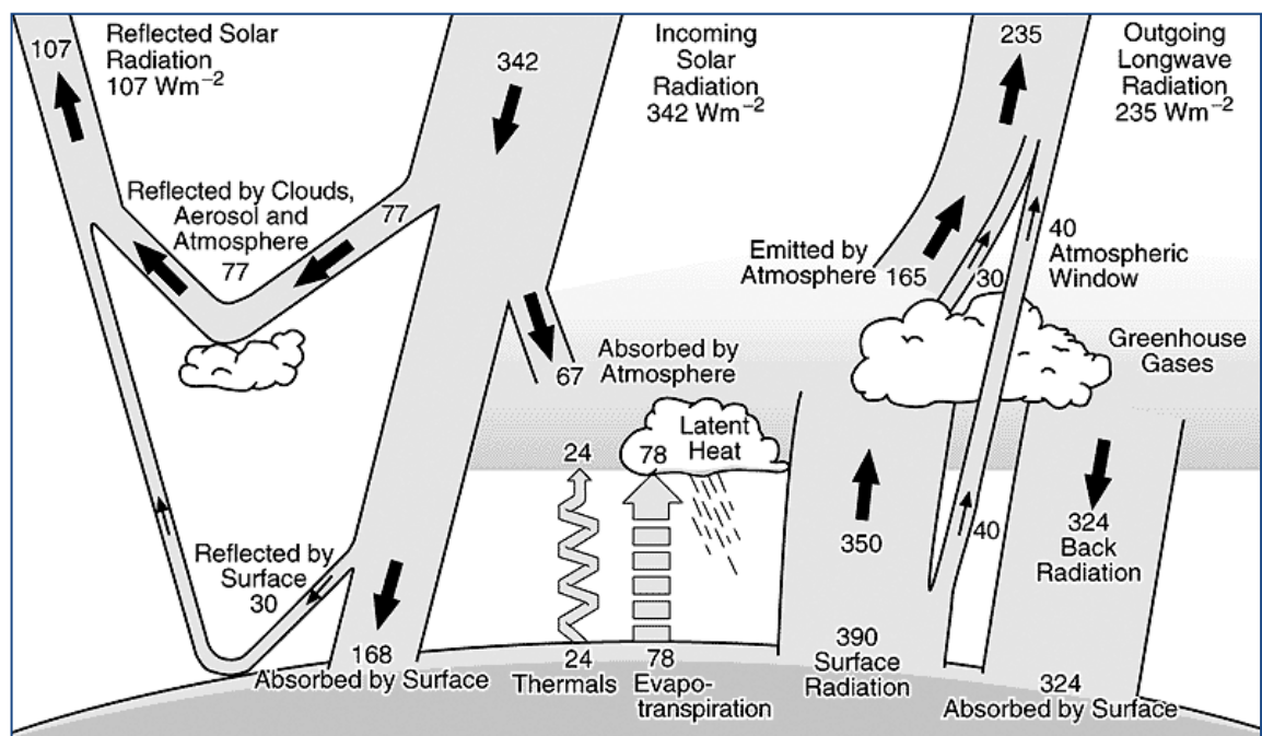
FIGURE 1.1 Energy flow in the global climate system
