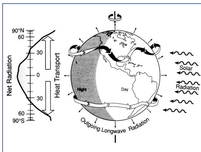
FIGURE 1.2 Net annual heating imbalance by latitude
