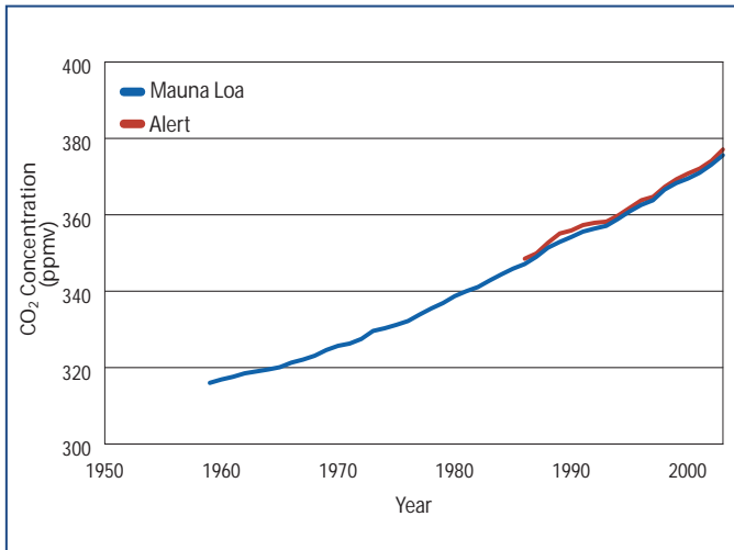
Atmospheric carbon dioxide concentrations since 1959
