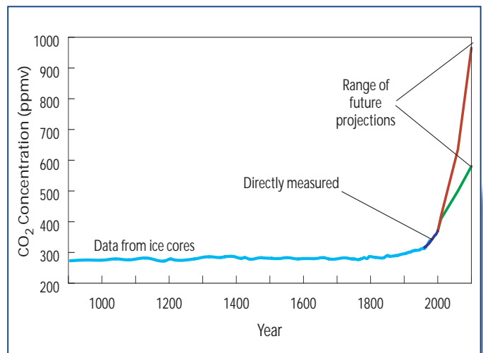
Projections for future atmospheric CO 2 concentrations, relative to concentrations of the past millennium
