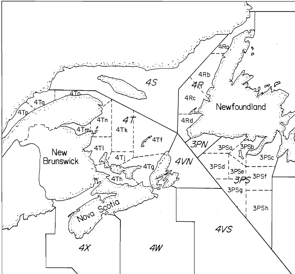
Figure 1. NAFO divisions including the Canadian fisheries statistical unit areas for the divisions examined.
