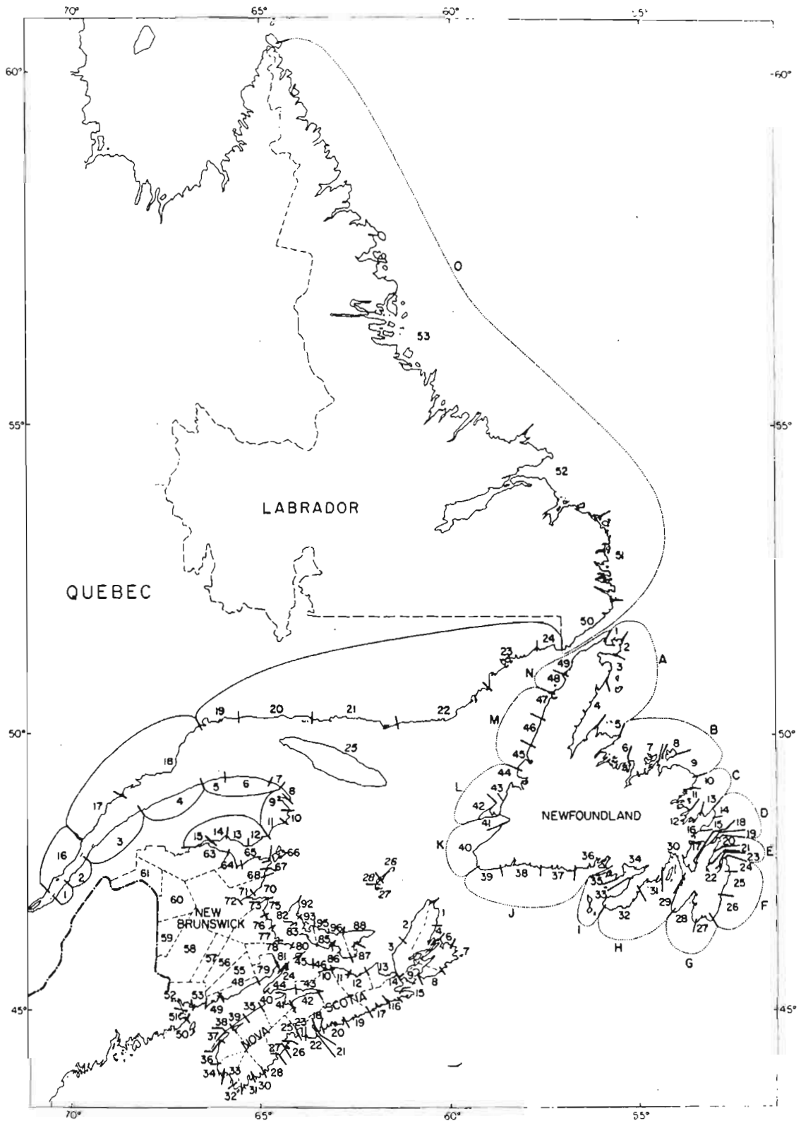
Figure 2. Fisheries statistical landing districts in the Maritimes, Quebec, and Newfoundland. See appendices A, B, and C.
