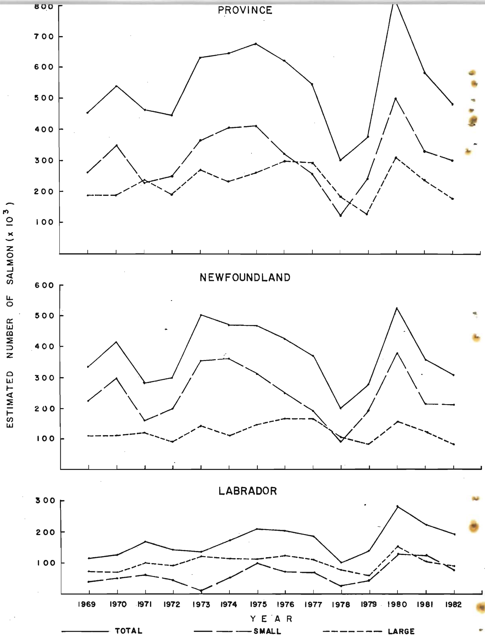
Fig. 5. The estimated number of salmon by size for 1969-82.
