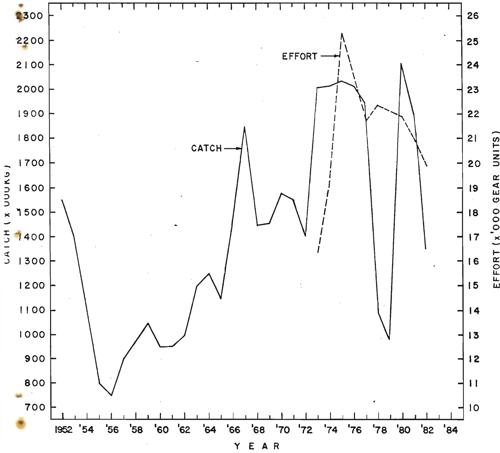
Fig. 4. Atlantic salmon commercial catch and effort data in Newfoundland and Labrador, 1952-82.
