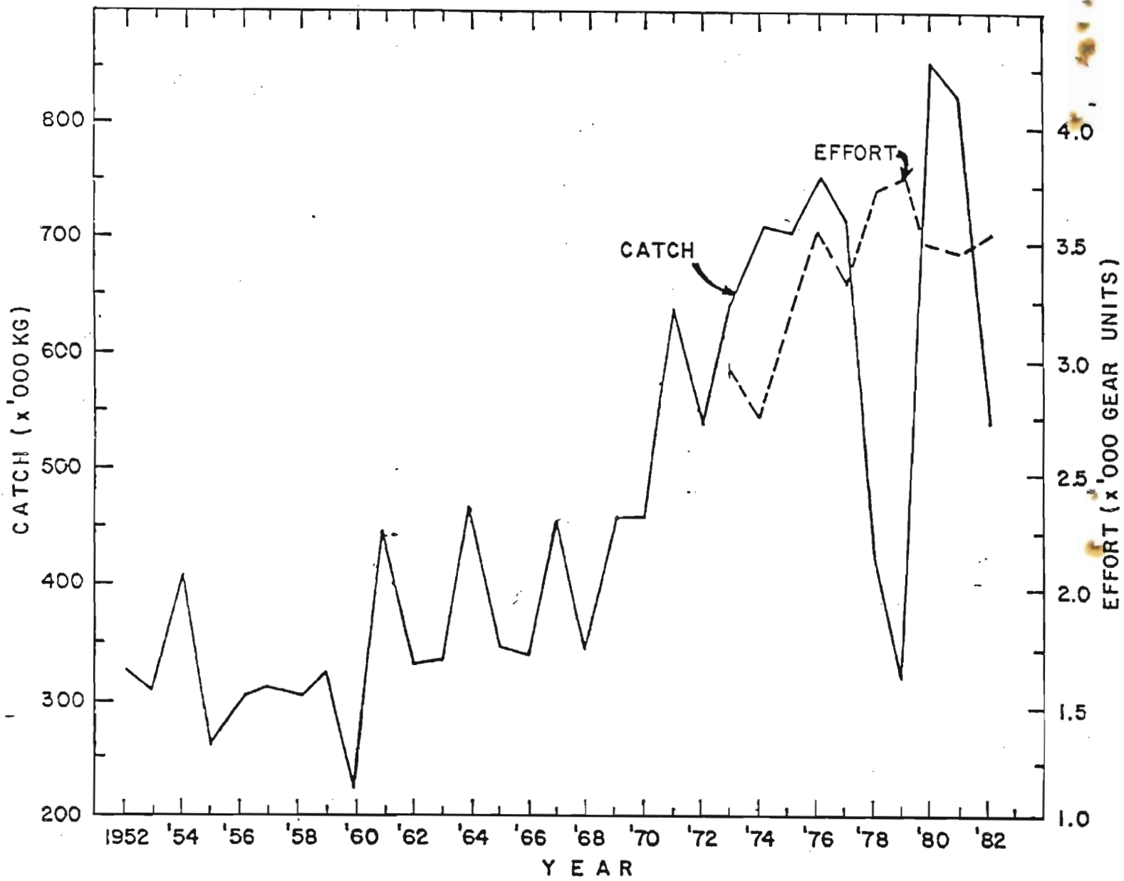
Fig. 7. Atlantic salmon commercial catch and effort data for Labrador, 1952-82.
