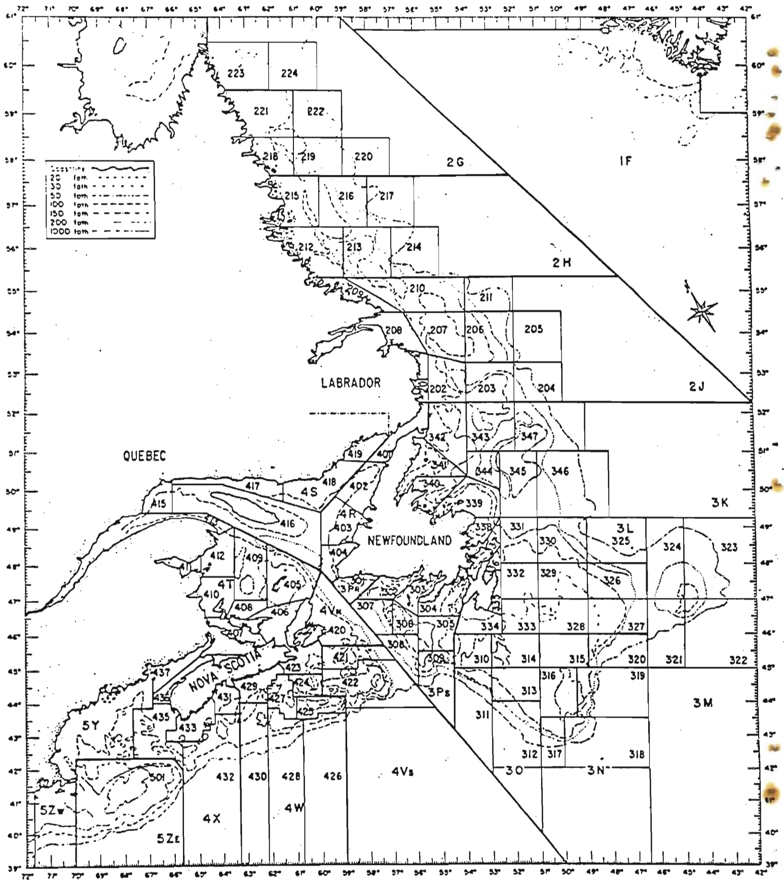
Fig. 3. ICNAF Divisions (2G-5Z) and Unit Areas (218-501).
