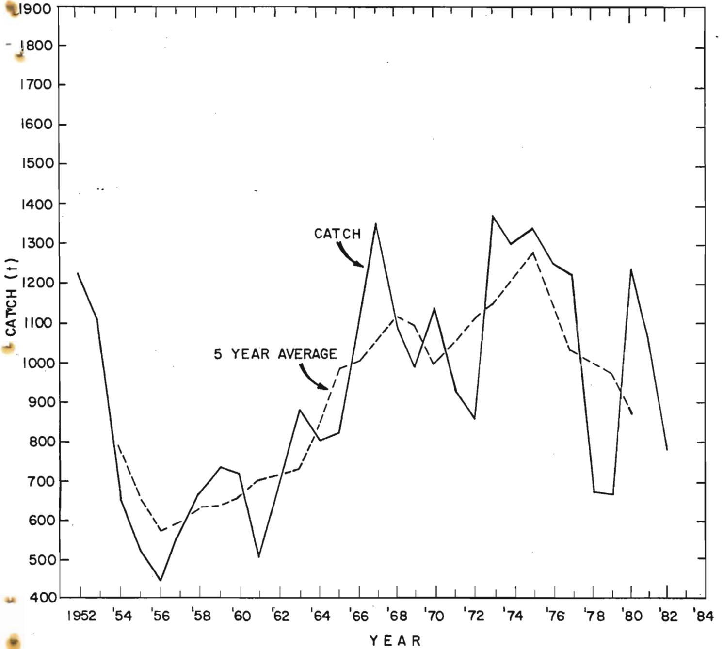
Fig. 6. Catches in the Atlantic salmon commercial fishery for insular Newfoundland, 1952-82.
