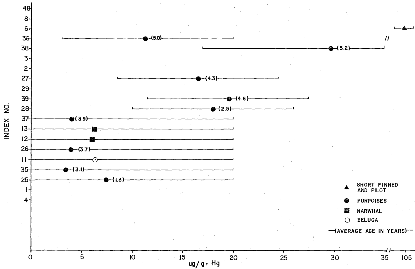
Figure 1. Mercury in liver of cetaceans.
