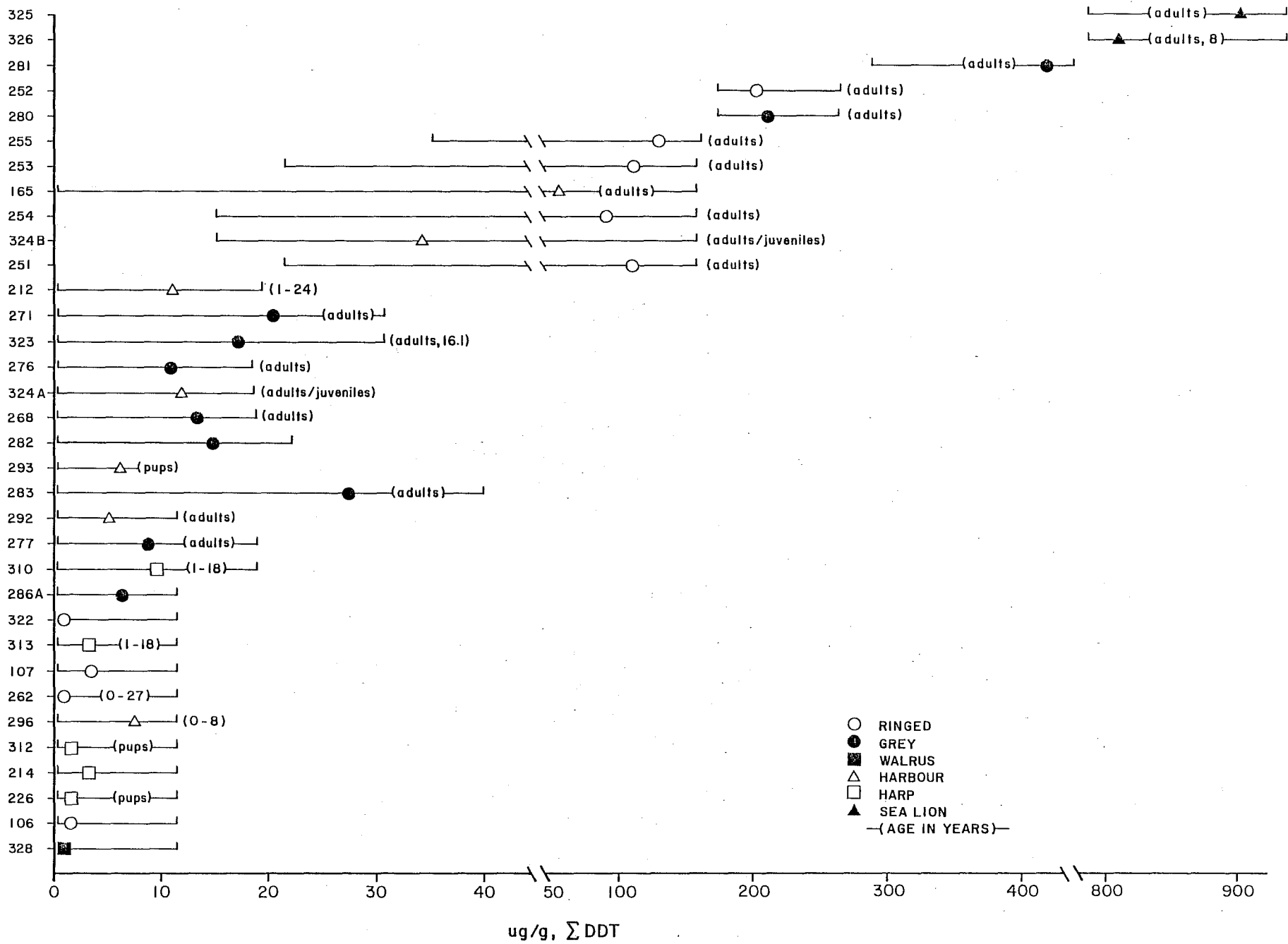
Figure 9. \Sigma DDT in pinnipeds (blubber).
