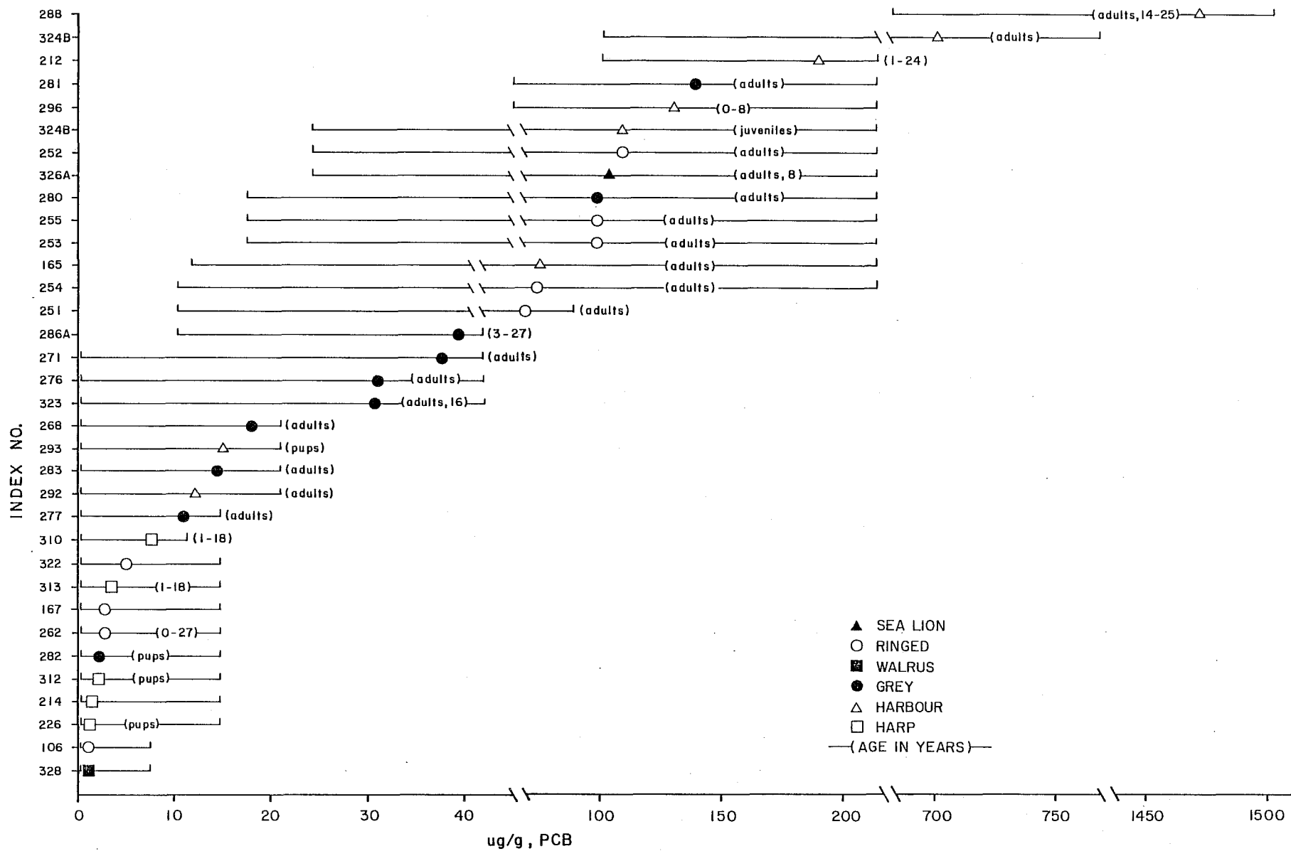
Figure 10. PCB in pinnipeds (blubber).
