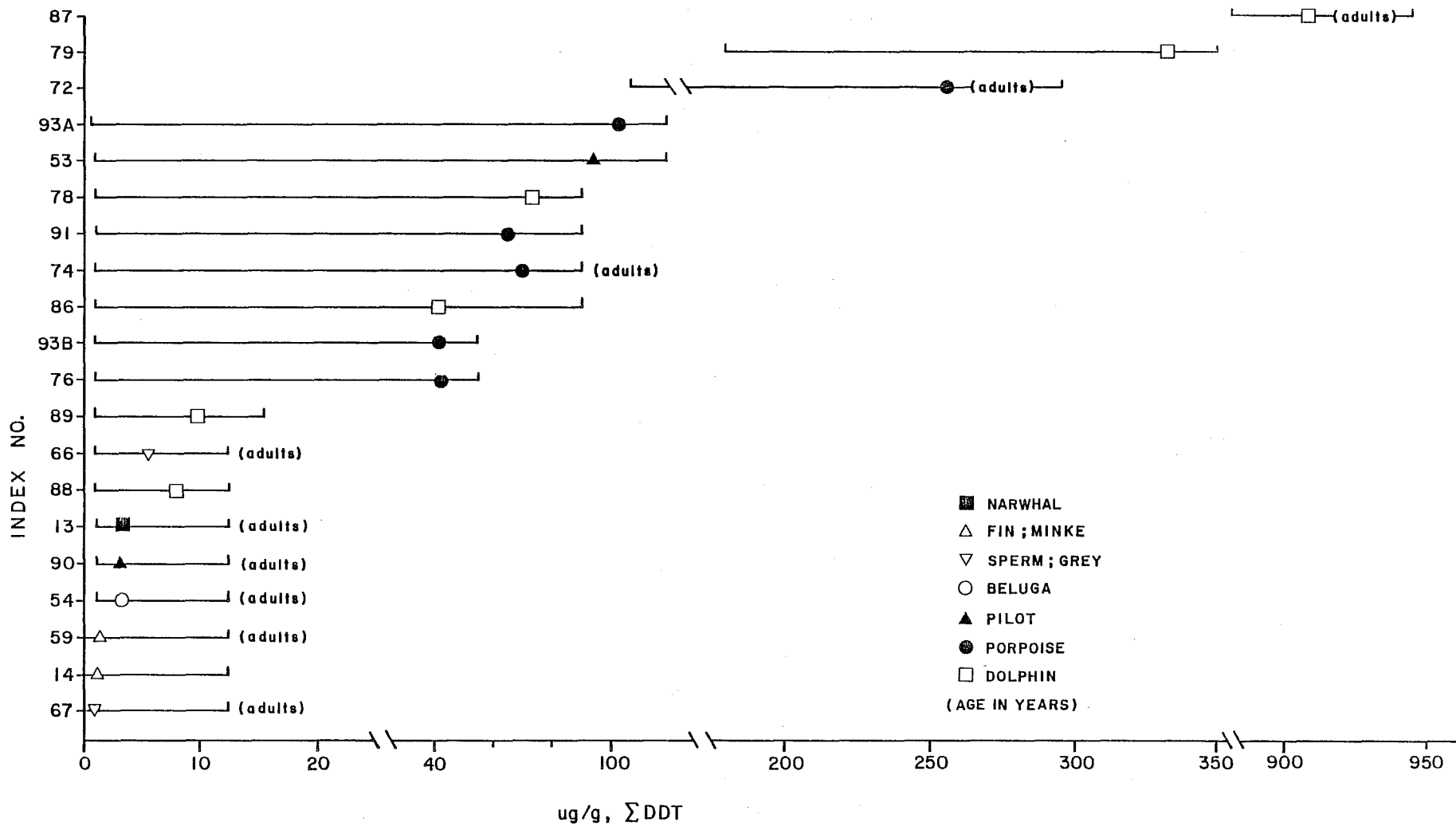
Figure 8. \Sigma DDT in cetaceans (blubber).
