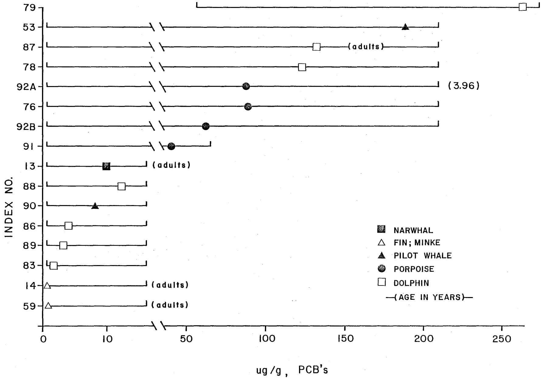
Figure 7. PCB's in cetaceans (blubber).
