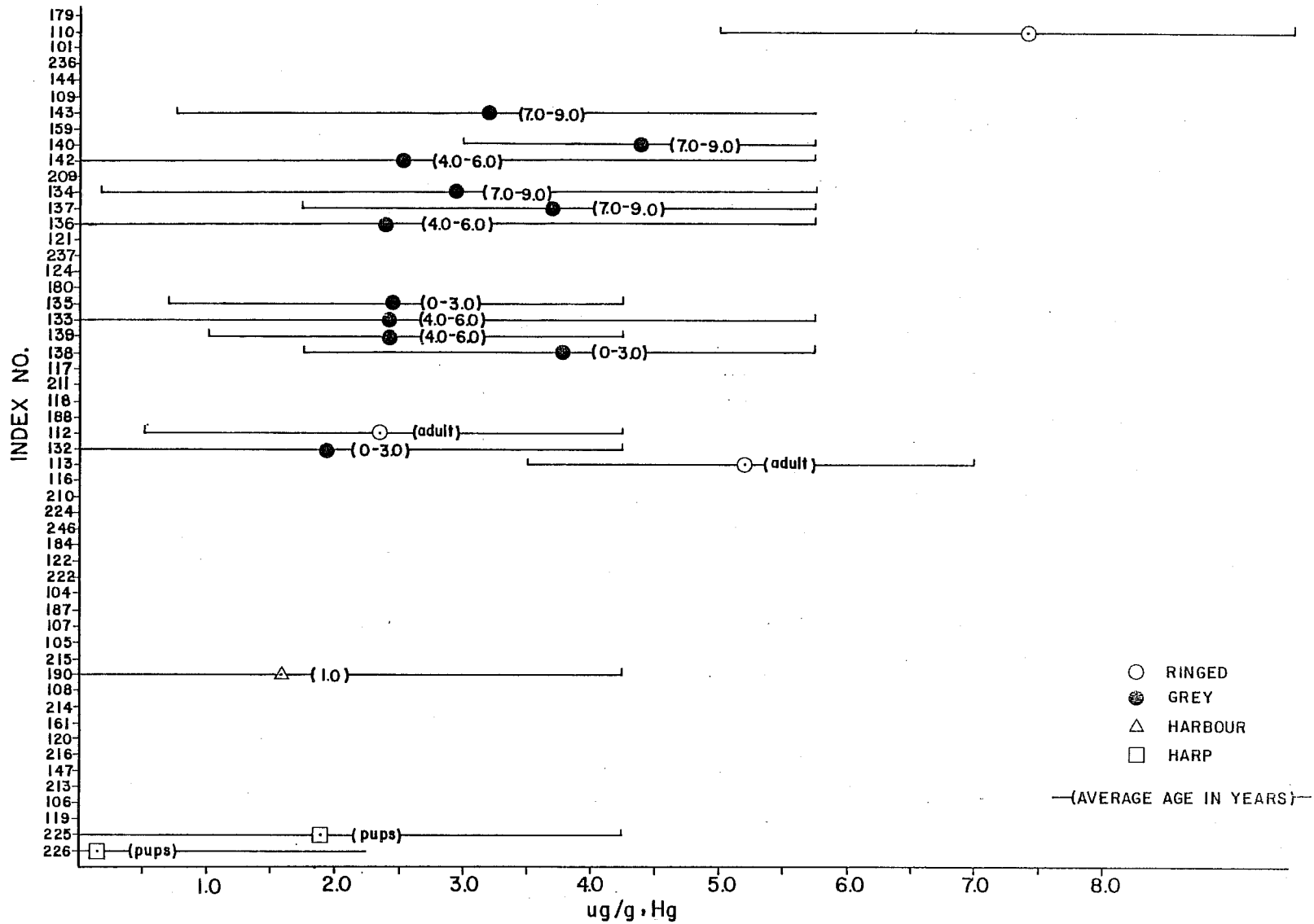
Figure 6. Mercury in kidney of seals.
