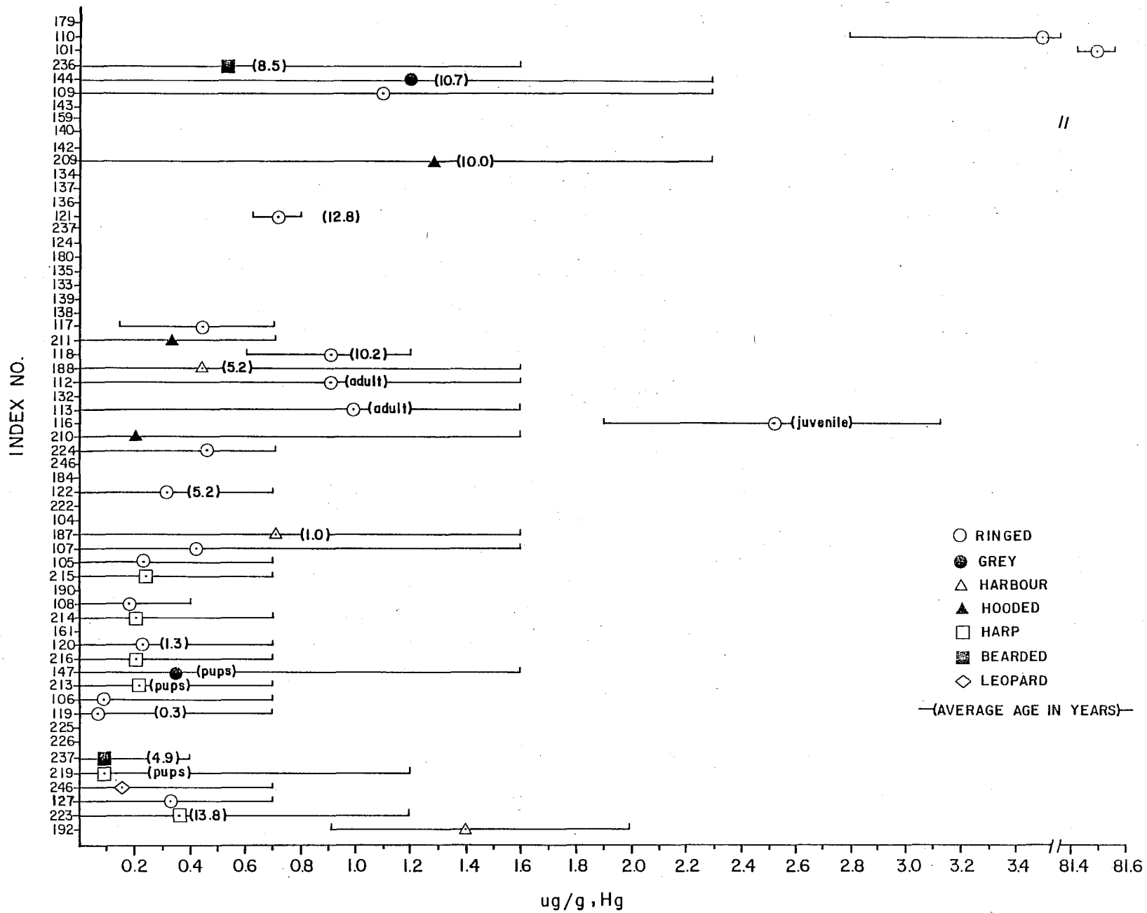
Figure 5. Mercury in muscle of seals.
