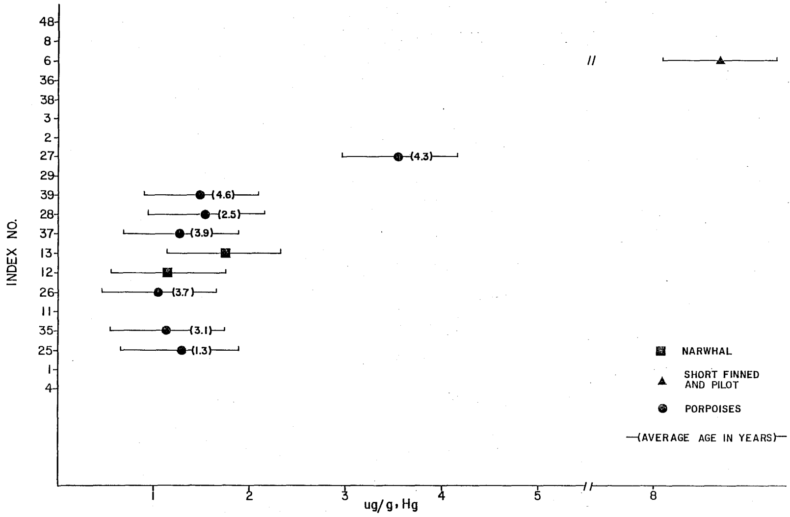
Figure 3. Mercury in kidney of cetaceans.
