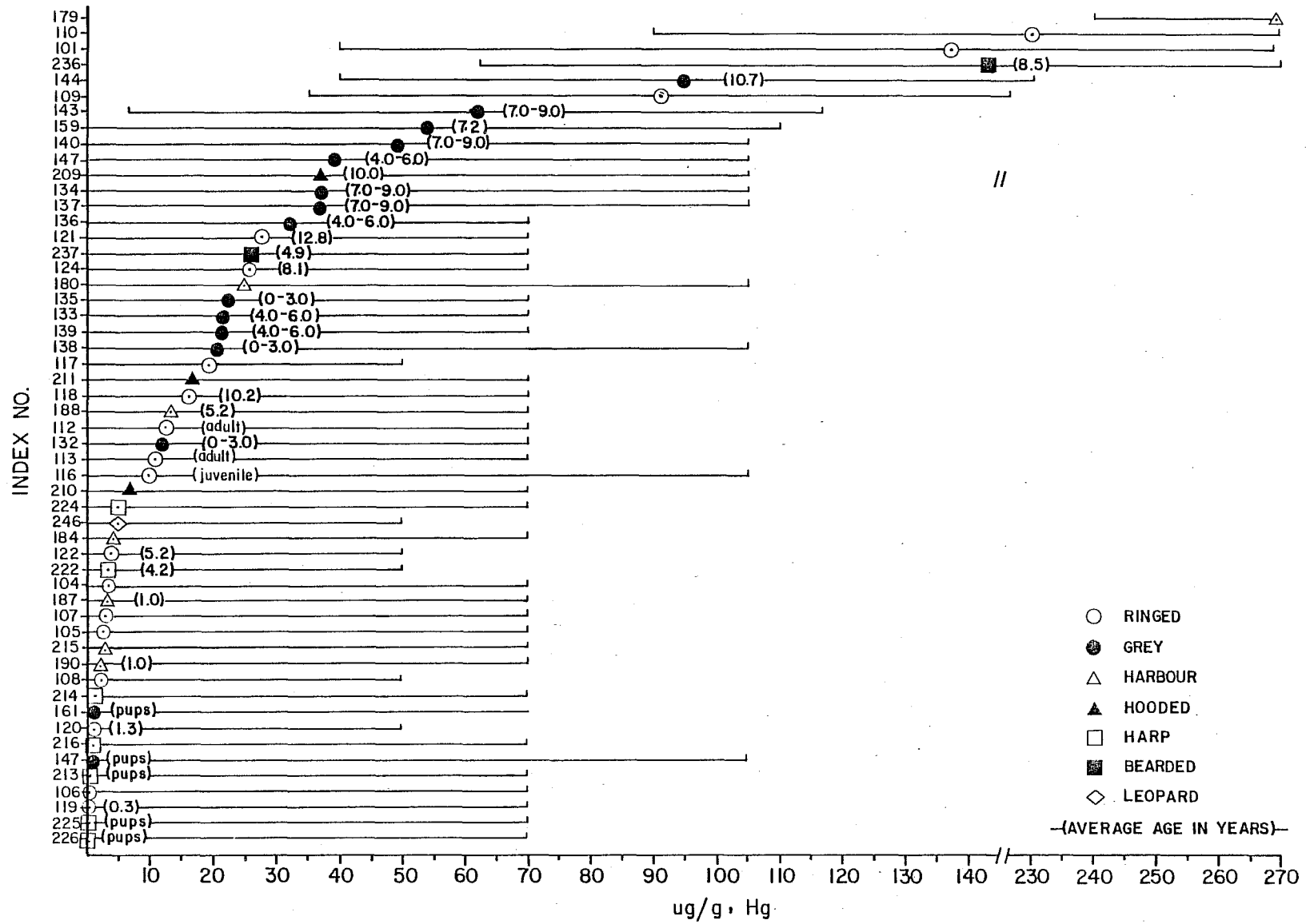
Figure 4. Mercury in liver of seals.
