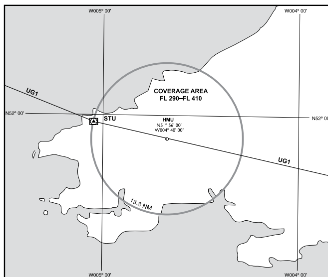
Figure 11.3—Strumble HMU
