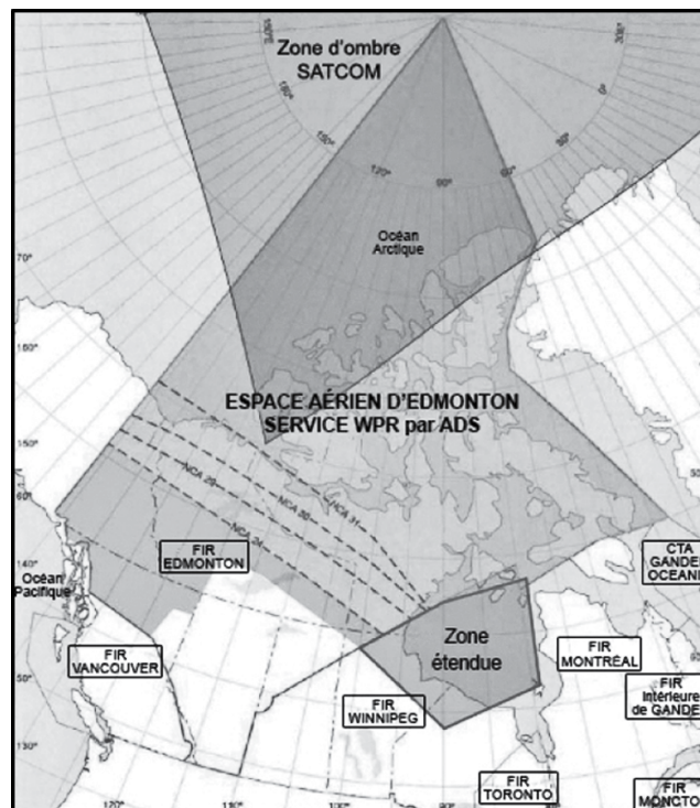
Figure 8.1 – Zone d'ombre SATCOM
