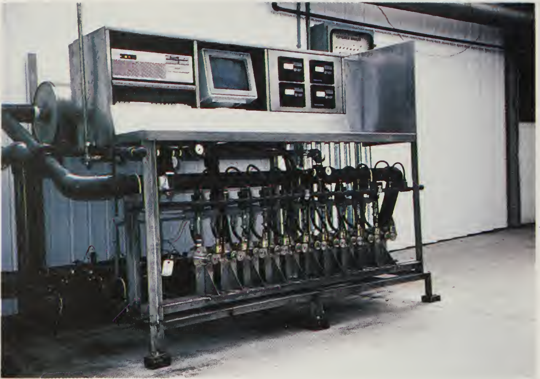
Plate II The Harrow Fertigation Manager® (HFM®), a computerized multifertilizer injection system (U.S. Patent #5 184 420) for the precise application of water and nutrients according to the changing needs of various crops. (Harrow Fertigation Manager® and HFM® are registered trade marks of Labbate Climate Control Systems Inc., 509 Hwy #77, R.R. #5, Leamington, Ont.)
