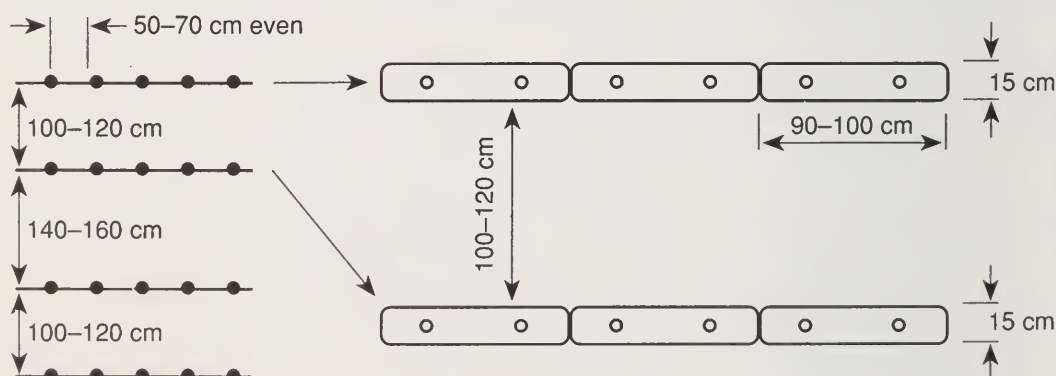
Fig. 15 Typical layout of plants for rock-wool culture. Option 1 : Plants are trained to the canopy system giving each plant about 50 \text{ cm} \times 160 \text{ cm} = 0.8 \text{ m}^2 . Option 2 : Plants are trained to the vertical cordon system giving each plant about 60 \text{ cm} \times 130 \text{ cm} = 0.78 \text{ m}^2 .
