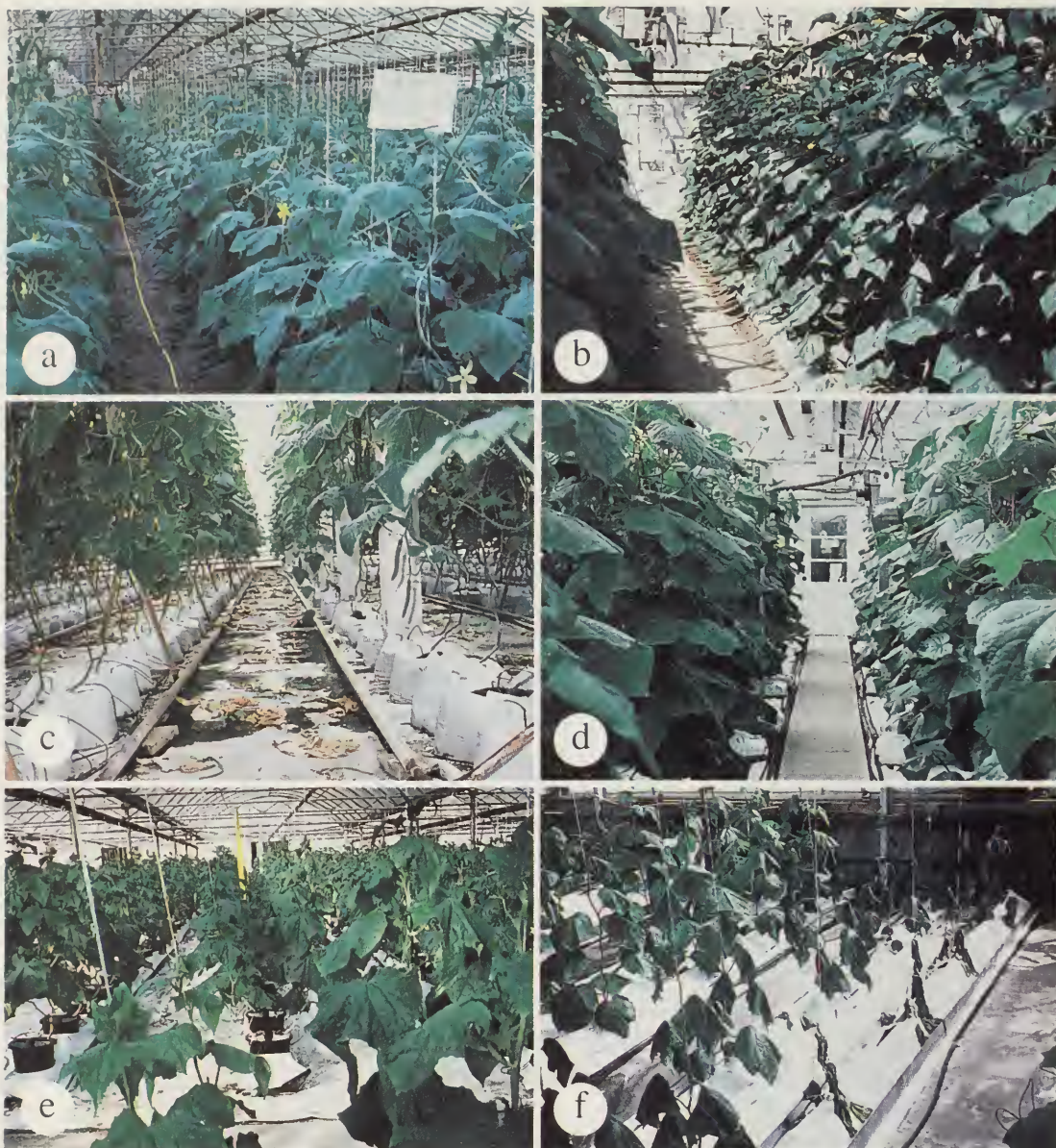
Plate IV Cropping of greenhouse seedless cucumbers in soil and soilless media:
