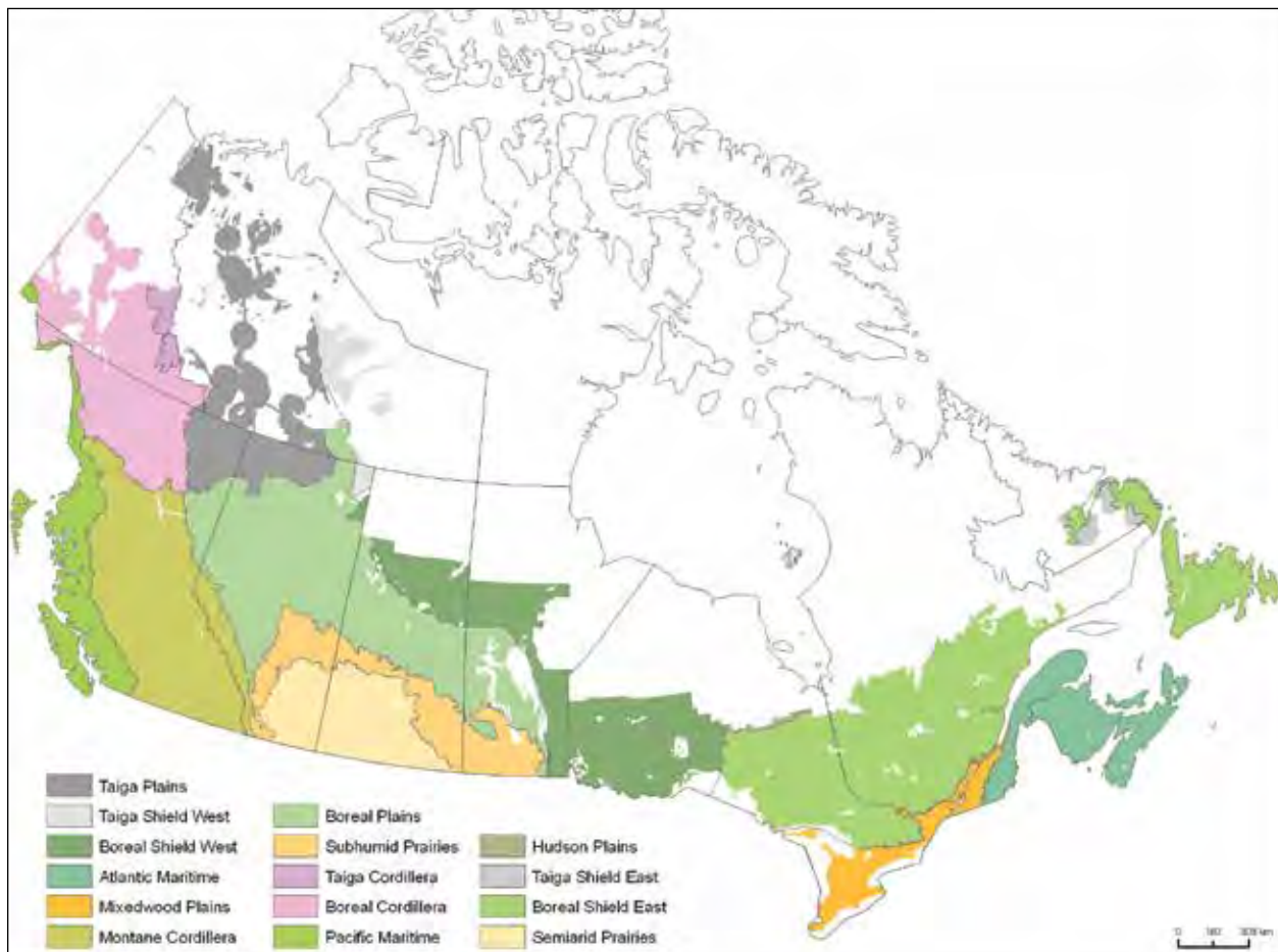
Figure 3-15. The terrestrial ecozones of Canada as used in the CBM-CFS3.
