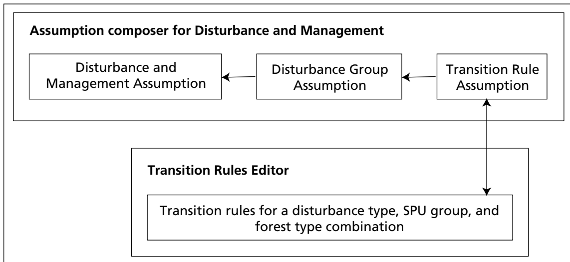
Figure 6-26. Links between the Assumption Composer for Disturbance and Management and the “Transition Rules Editor”.
