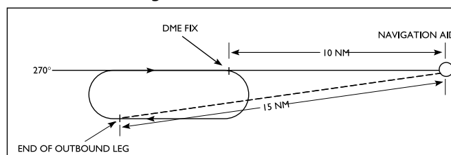
Figure 10.4 –DME Hold
