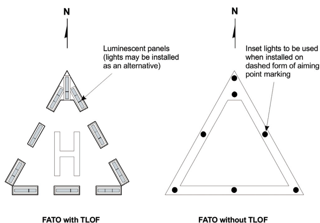
Aiming point lighting
