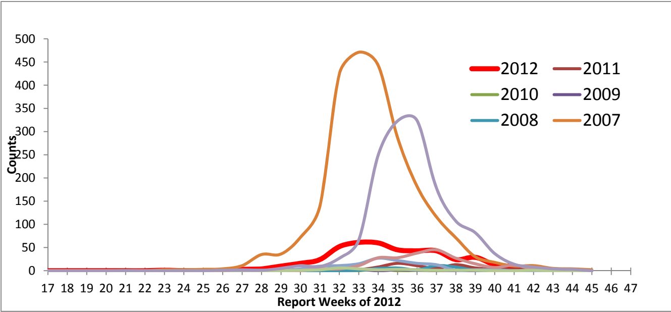
WNV clinical cases and asymptomatic infections by report week, 2012 season compared to previous seasons
