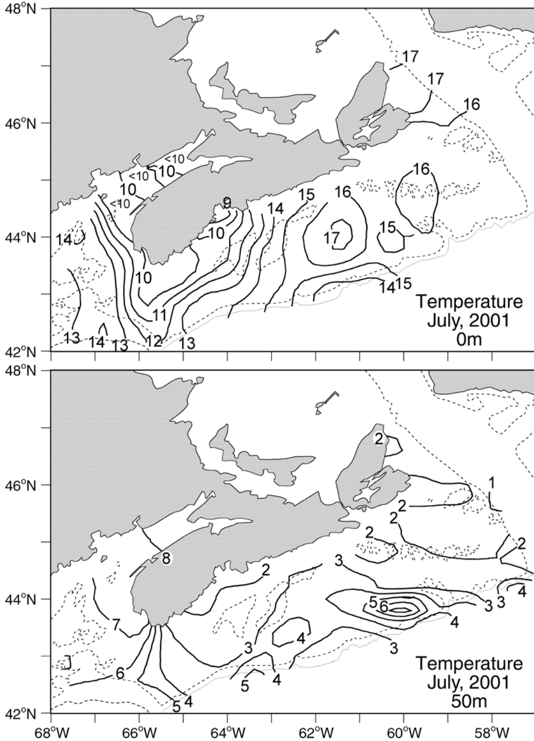
Fig.14a. Contours of temperatures at the surface (top panel) and 50 m (bottom panel) during the 2001 July groundfish and ITQ surveys.
