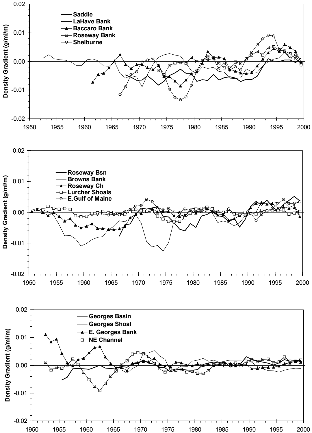
Fig.24b. Five-yr running means of the annual anomalies of the density gradient between the surface and 50 calculated for the areas 16-29 in Fig. 8.
