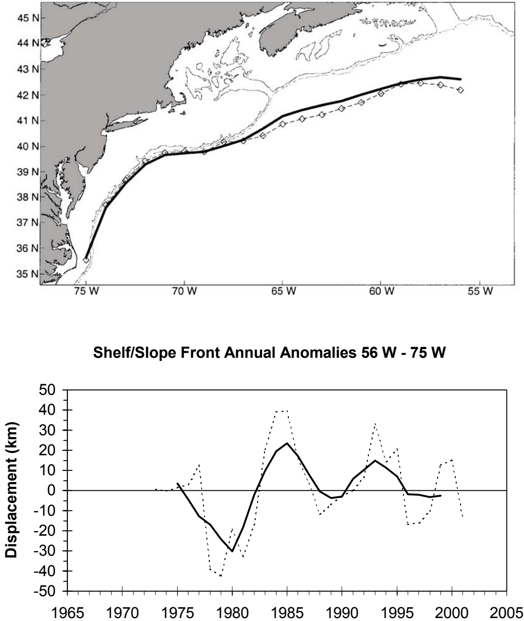
Fig.25. The 2001 (dashed line) and long-term mean (1973-2000; solid line) positions of the shelf/slope front (top panel) and the time series of the annual anomaly of the mean (56°-75°W) position of the shelf/slope front (bottom panel).
