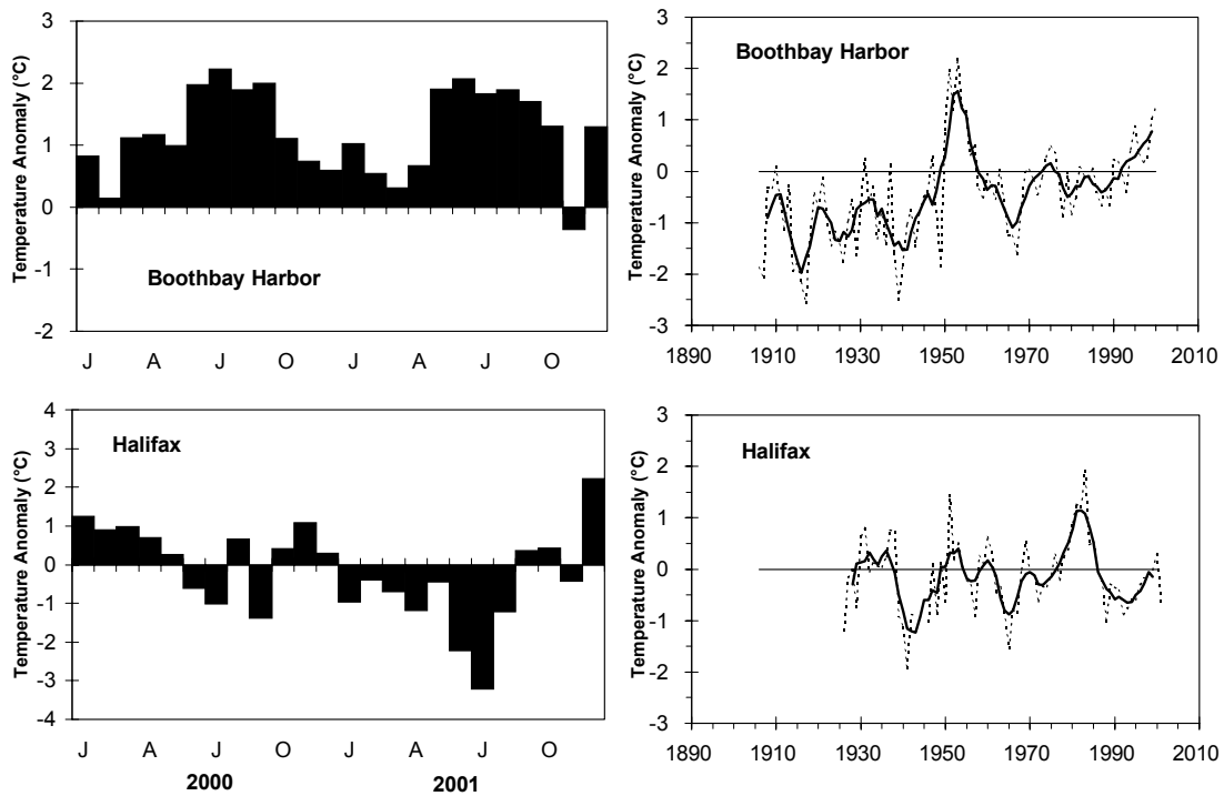
Fig. 2. The monthly sea surface temperature anomalies during 2000 and 2001 (left) and the annual temperature anomalies (dashed line; right) and their 5-year running means (solid line; right) for Boothbay Harbor (top panels) and Halifax Harbour (bottom panels). Anomalies are relative to the 1971-2000 means.
