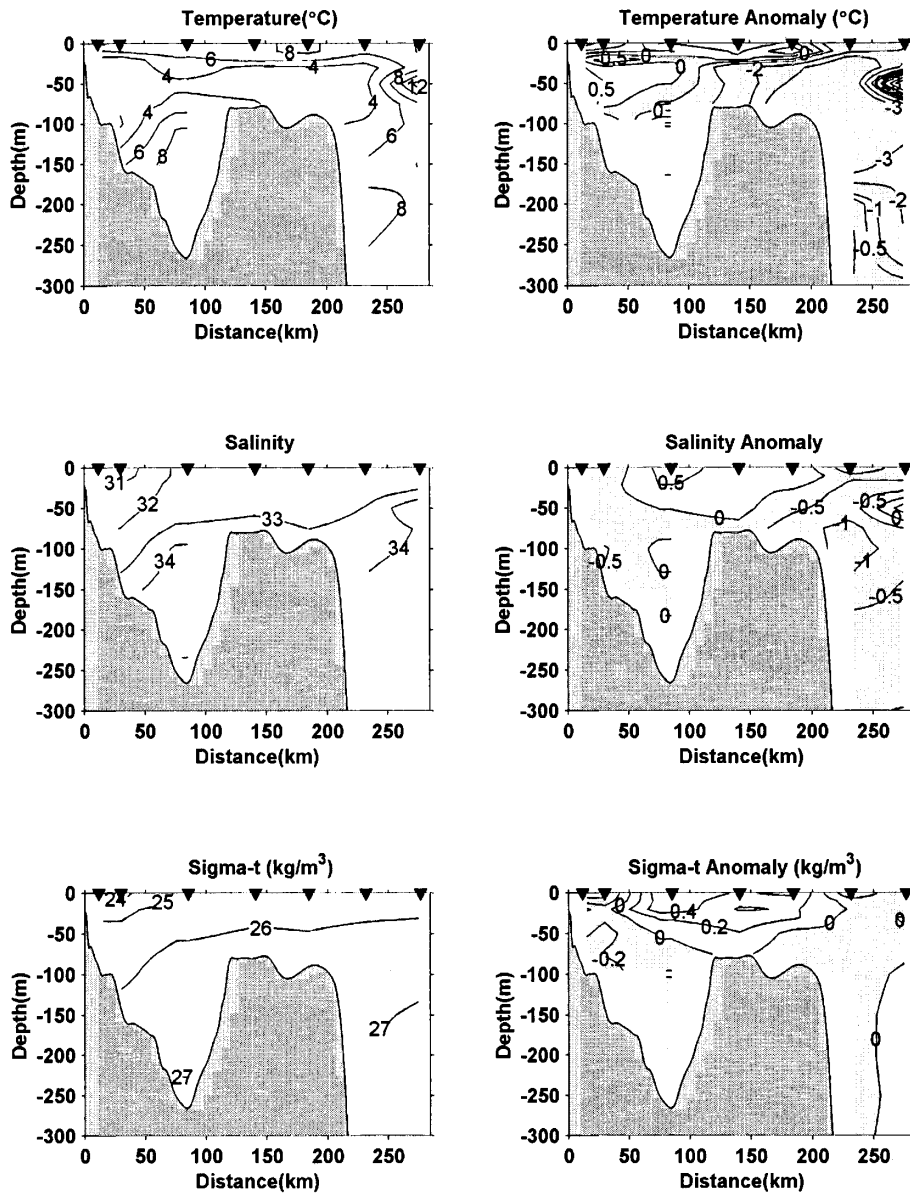
Fig.20. Contours of the temperature, salinity and sigma-t (left panels) and their anomalies (right panels) along the Halifax Line during 31 May-1 June 2001 (left panels). The triangles denote the location of the standard stations.
