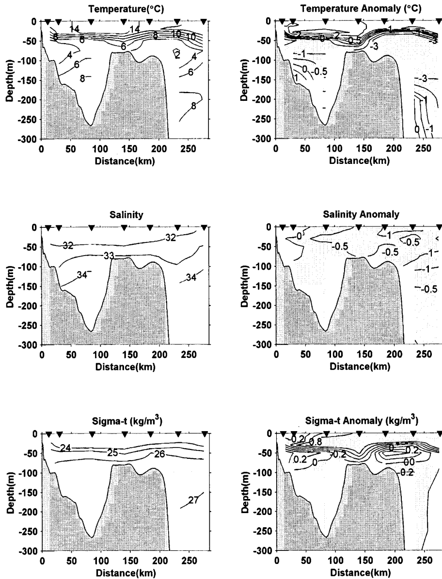
Fig.21. Contours of the temperature, salinity and sigma-t (left panels) and their anomalies (right panels) along the Halifax Line during October 2001 (left panels). The triangles denote the location of the standard stations.
