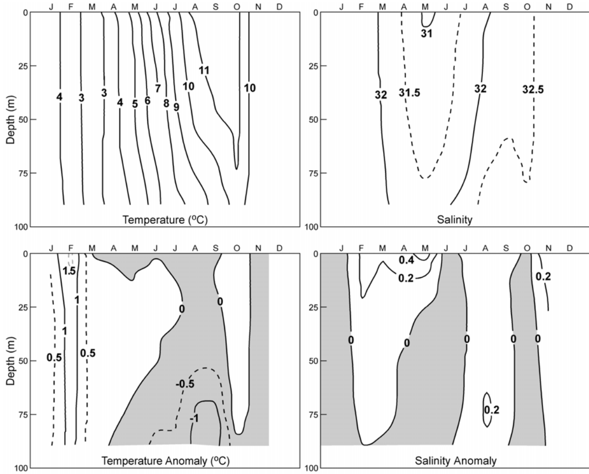
Fig. 3. Contours of monthly mean temperature (left) and salinity (right) and their anomalies (bottom panels) at Prince 5 as a function of depth during 2001 relative to the 1971-2000 means. Colder and fresher-than-normal conditions are shaded.
