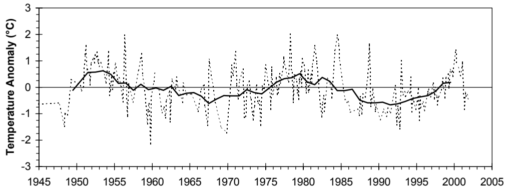
Fig.10. 2001 monthly temperature anomaly profiles (top 2 panels) plus the monthly mean temperature anomaly time series (dashed line) and the 5-yr running mean of the estimated annual anomalies (solid line) at 100 m (bottom panel) for Misaine Bank (area 5-Fig. 8).
