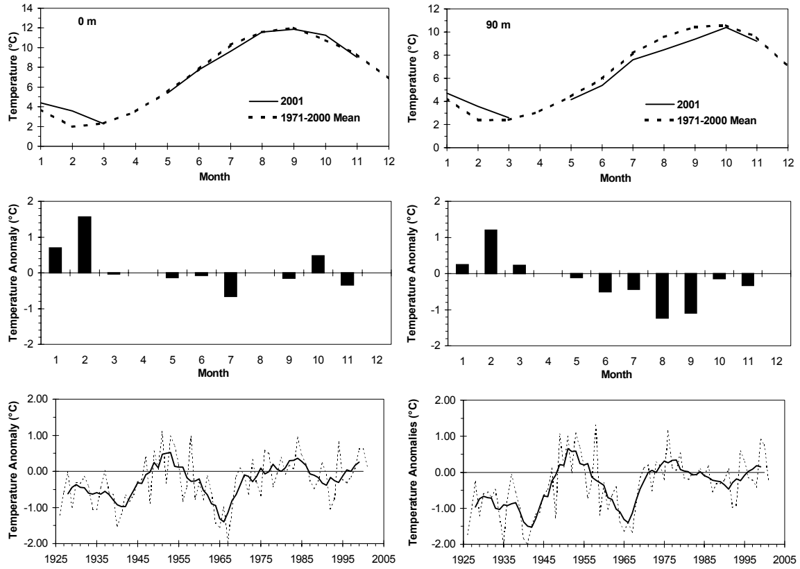
Fig. 4. The monthly mean temperatures for 2001 (solid line; top panels) and their long-term means (dashed line; top panels), the monthly anomalies relative to the long-term means for 1971-2000 (middle panels) and in the bottom panels are the time series of the annual means (dashed lines) and their 5-year running means (solid line) for Prince 5, 0 m (left) and 90 m (right).
