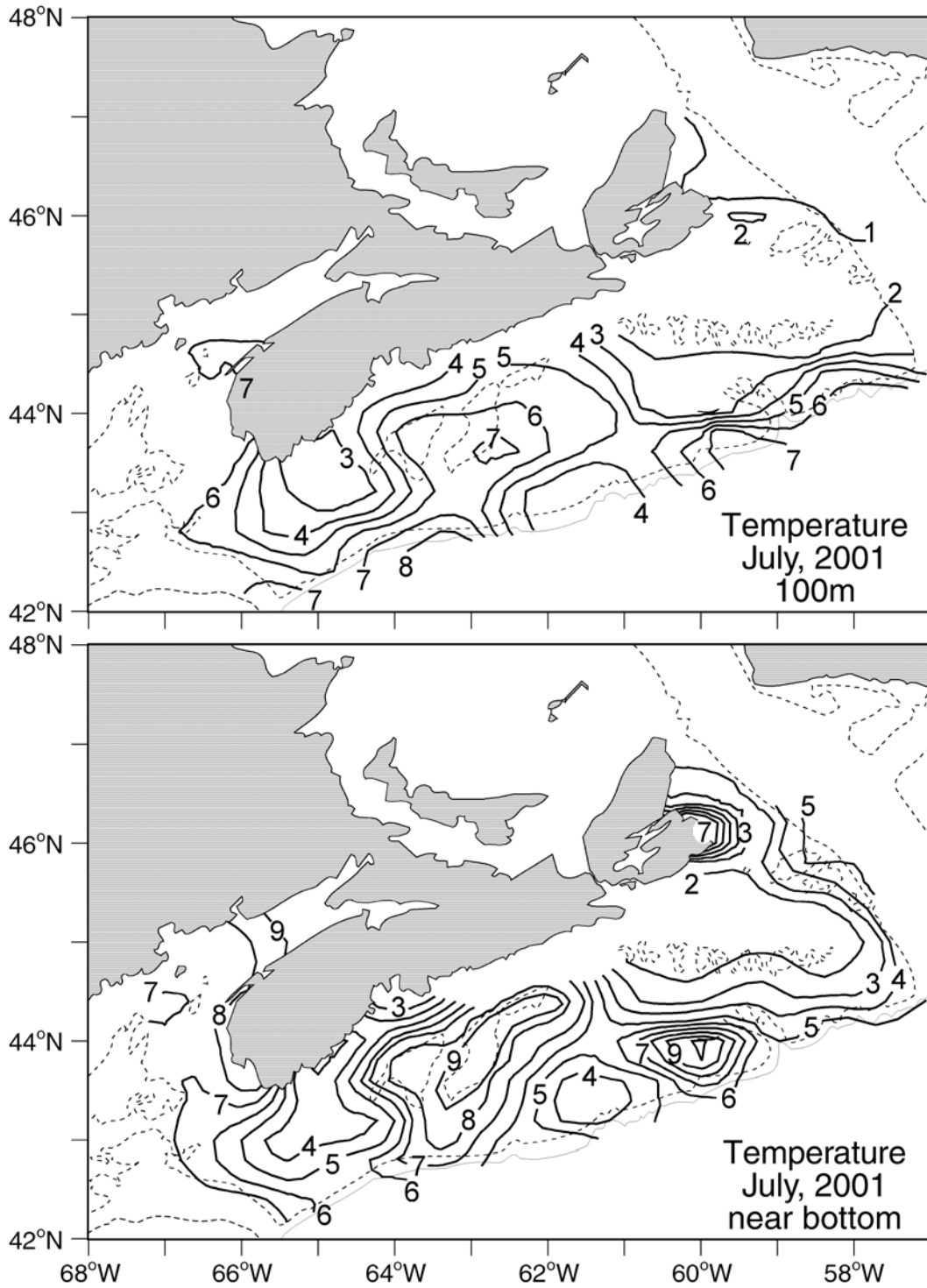
Fig.14b. Contours of temperatures at 100 m (top panel) and near bottom (bottom panel) during the 2001 July groundfish and ITQ surveys.
