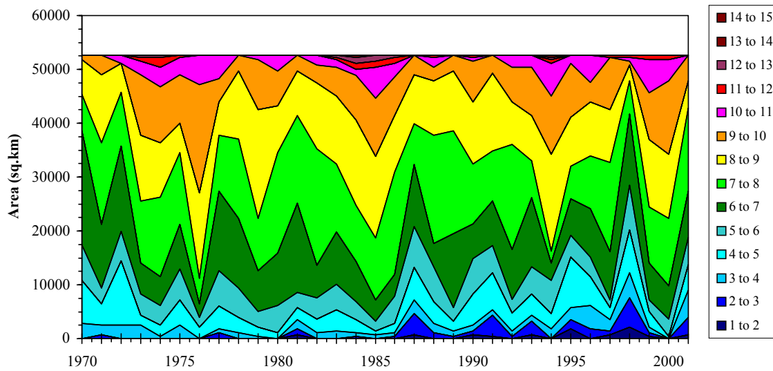
Fig.16b. The time series of the area of the bottom for each 1 degree temperature range for NAFO Subareas 4W (top panel) and 4X(bottom panel).
