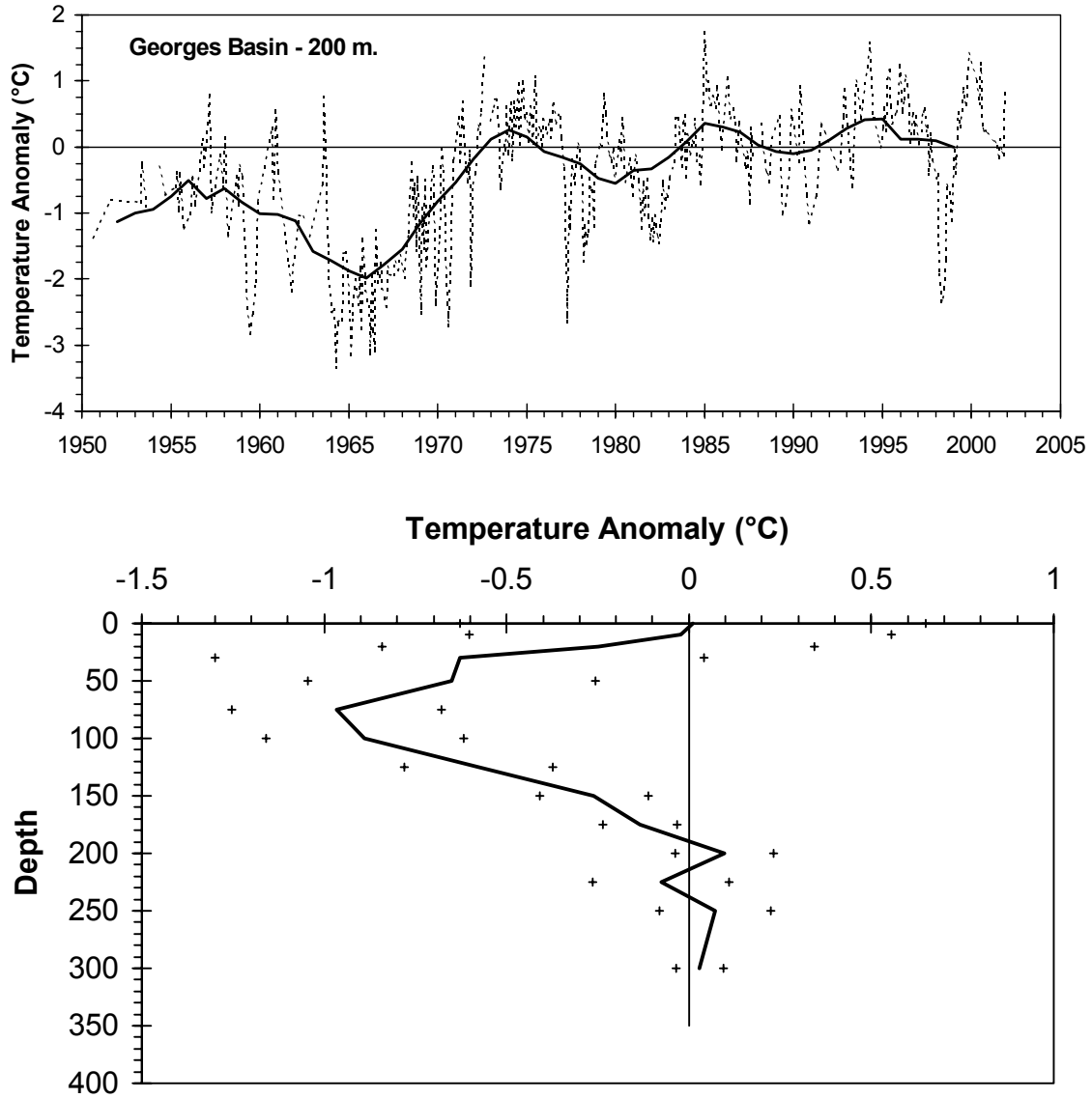
Fig.12. Time series of available monthly mean temperature anomalies at 200 m in Georges Basin (dashed line) and their 5-year running means (solid line) in the top panel. The bottom panel shows the annual temperature anomalies for 2001 as a function of depth. The crosses represent standard error of the means based upon the available monthly anomalies.
