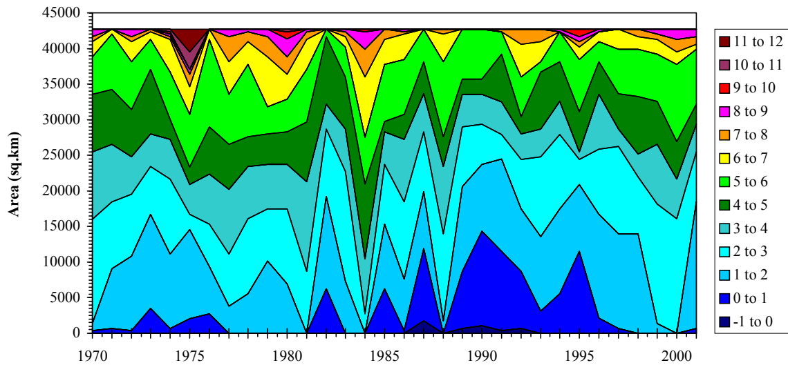
Fig.16a. The time series of the area of the bottom for each 1 degree temperature range for NAFO Subareas 4Vn (top panel) and 4Vs(bottom panel).
