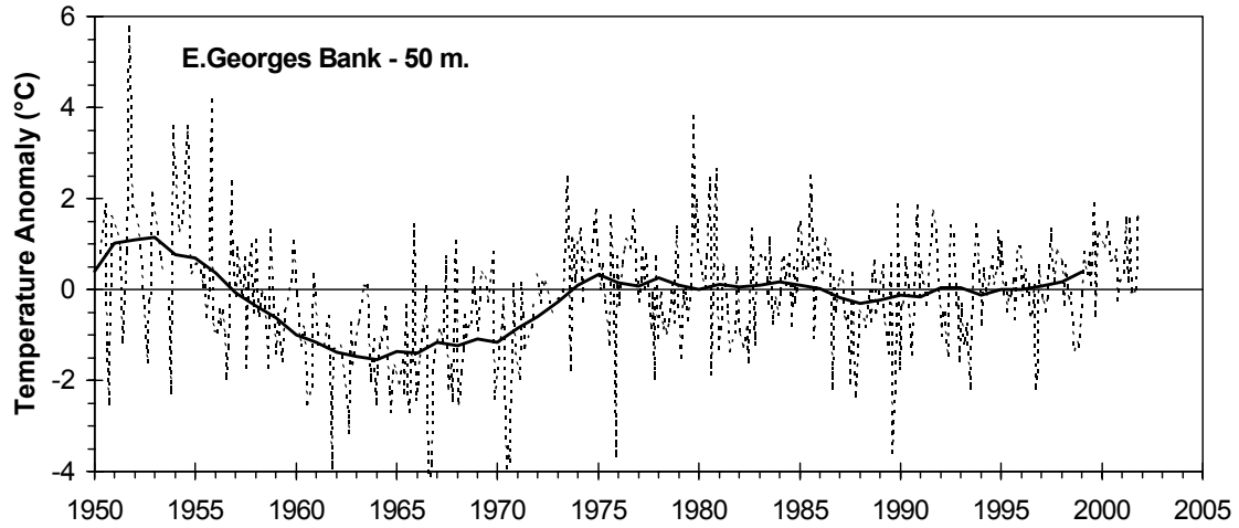
Fig.13. Time series of monthly mean temperature anomalies at 50 m on eastern Georges Bank (dashed lines) and their 5-year running means (solid line).
