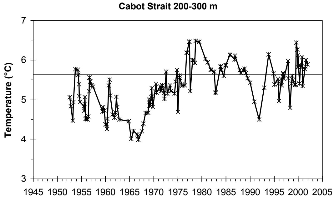
Fig.17. Average temperature over the 200-300 m layer in Cabot Strait. The horizontal line indicates the long-term mean during 1971-2000.
