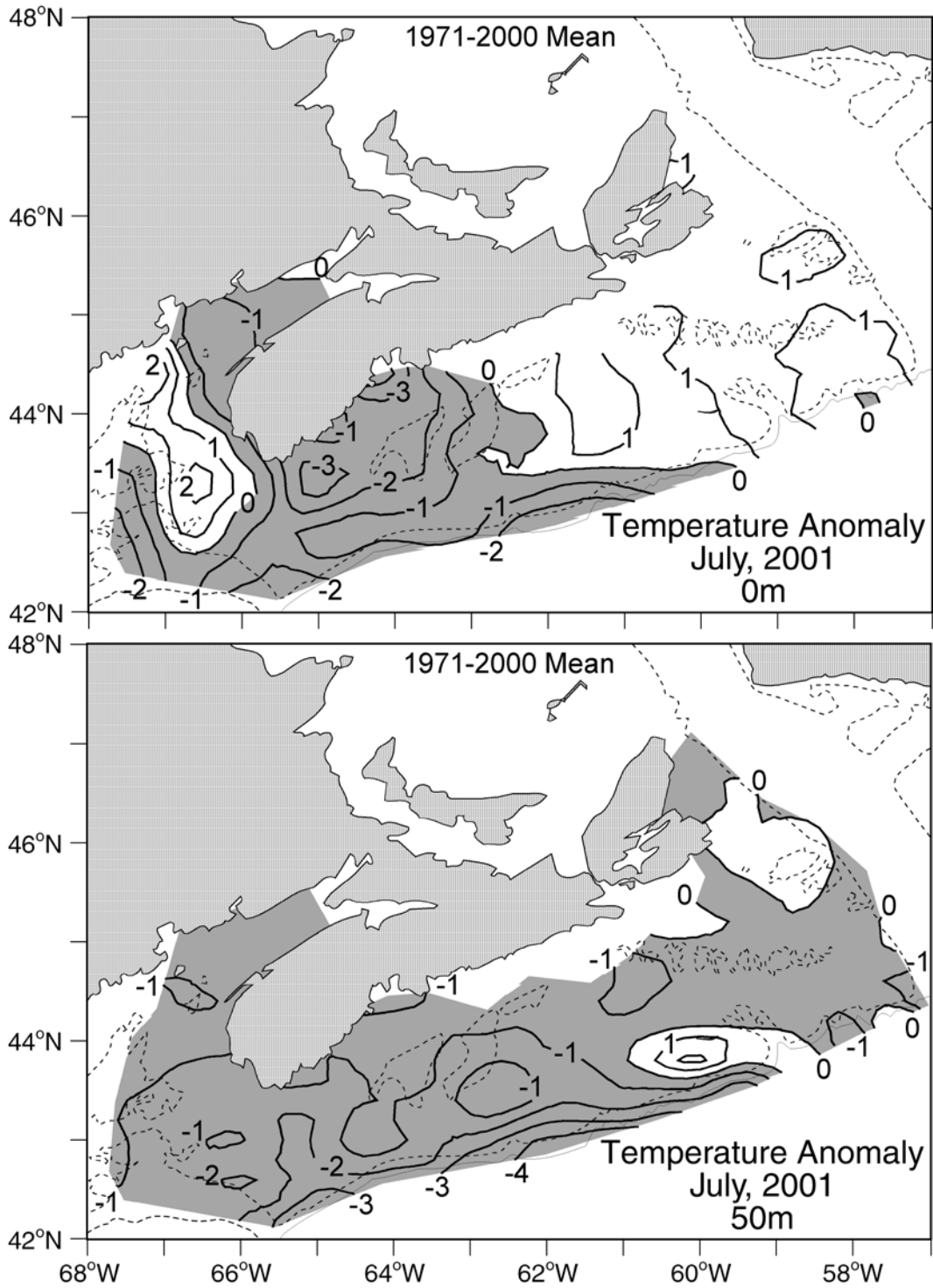
Fig. 15a. Contours of temperature anomalies at the surface (top panel) and 50 m (bottom panel) during the 2001 July groundfish and ITQ surveys.
