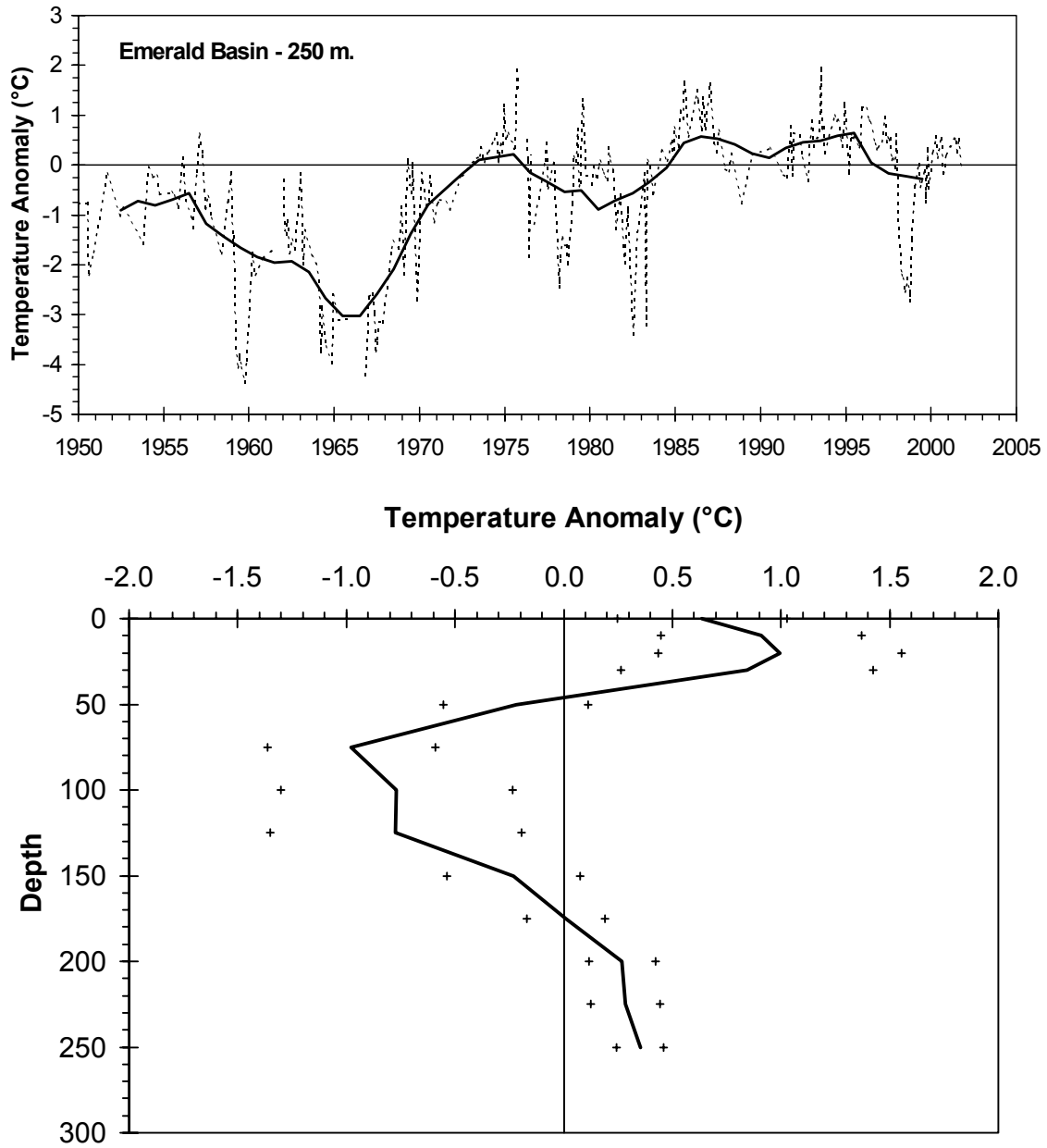
Fig. 7. Time series of available monthly mean temperature anomalies at 250 m in Emerald Basin (dashed line) and their 5-year running means (solid line) in the top panel. The bottom panel shows the annual temperature anomalies for 2001 as a function of depth. The crosses represent standard error of the means based upon the available monthly anomalies.
