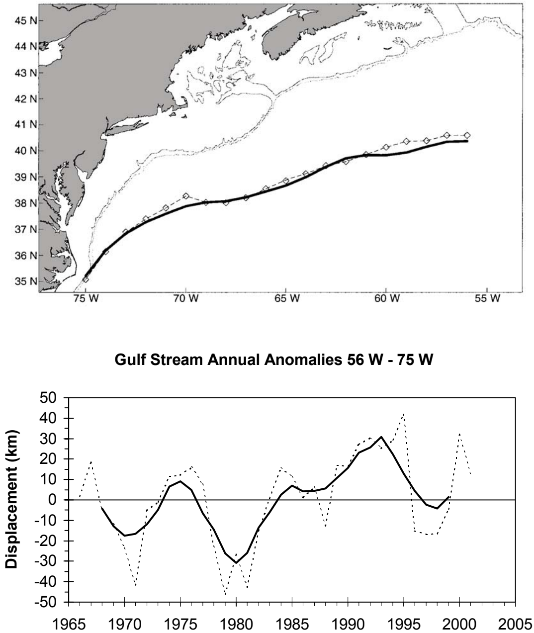
Fig.26. The 2001 (dashed line) and long-term mean (1973-2000; solid line) positions of the northern edge of the Gulf Stream (top panel) and the time series of the annual anomaly of the mean (56°-75°W) position of the Gulf Stream front (bottom panel).
