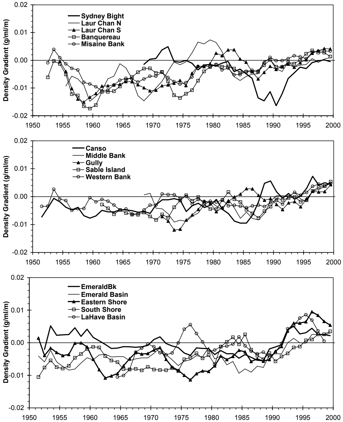
Fig.24a. Five-yr running means of the annual anomalies of the density gradient between the surface and 50 calculated for the areas 1-15 in Fig. 8.
