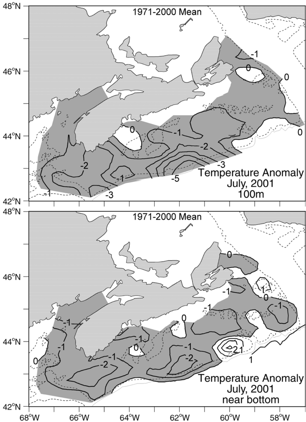
Fig.15b. Contours of temperature anomalies at 100 m (top panel) and near bottom (bottom panel) during the 2001 July groundfish and ITQ surveys.
