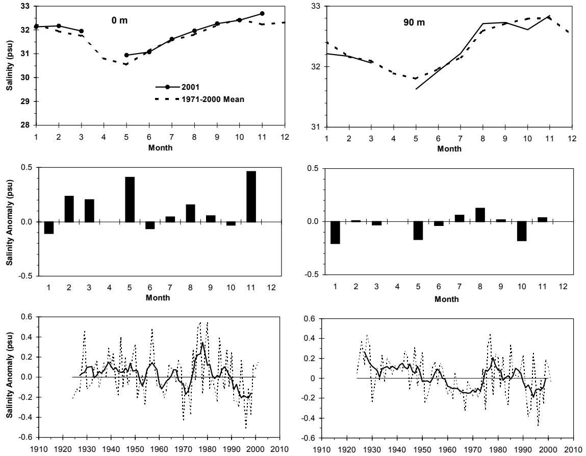
Fig. 5. The monthly mean salinities for 2001 (solid line; top panels) and their long-term means (dashed line; top panels), the monthly anomalies relative to the long-term means for 1971-2000 (middle panels) and in the bottom panels are the time series of the annual means (dashed lines) and their 5-year running averages (solid line) for Prince 5, 0 m (left) and 90 m (right).
