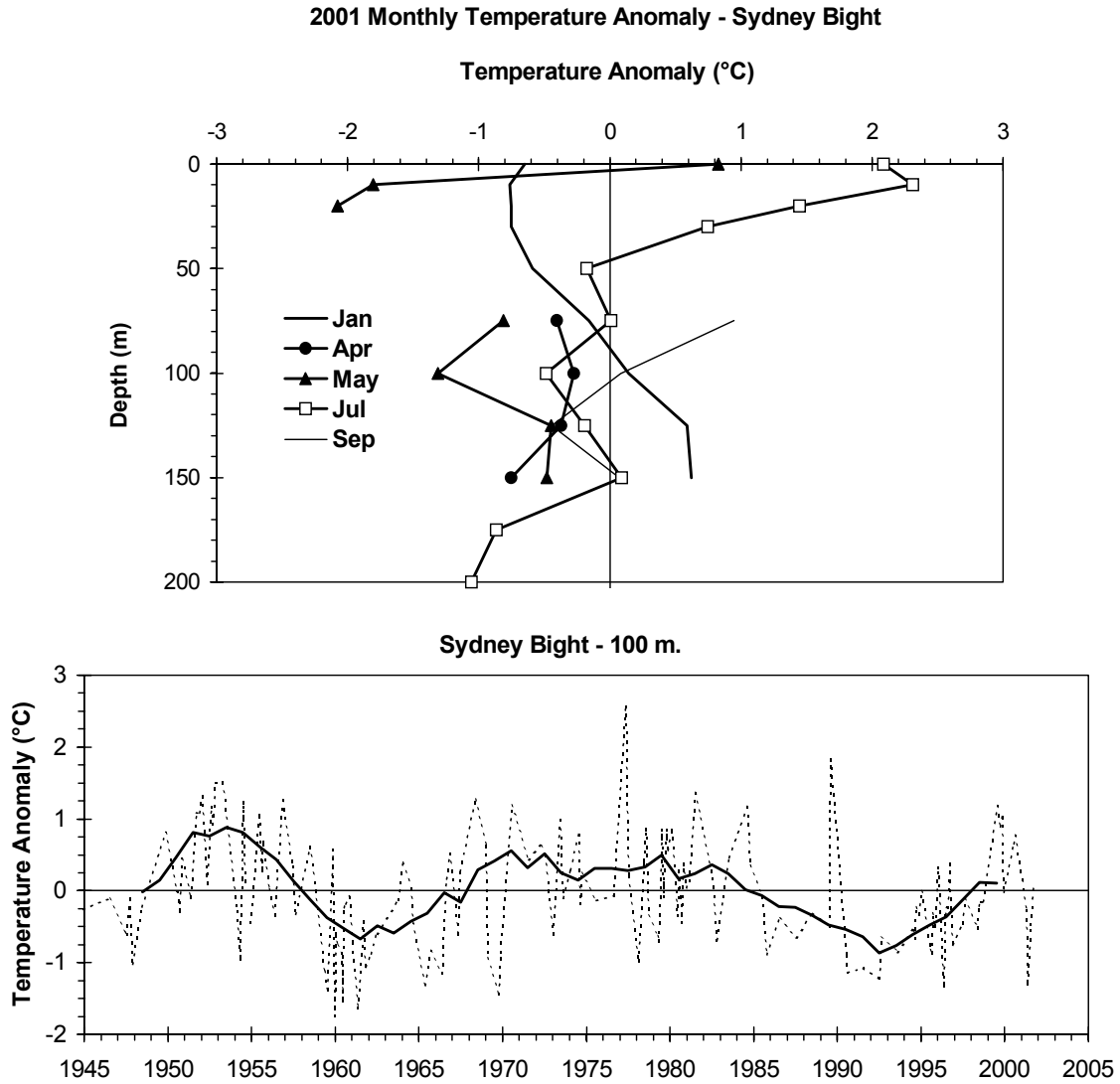
Fig. 9. 2001 monthly temperature anomaly profiles (top panel) plus the monthly mean temperature anomaly time series (dashed line) and the 5-yr running mean of the estimated annual anomalies (solid line) at 100 m (bottom panel) for Sydney Bight (area 1-Fig. 8).
