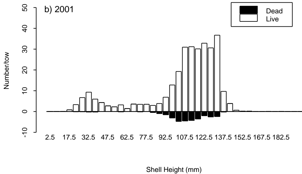
Fig. 13. Comparison of shell height frequencies from the 2000 and 2001 survey of Scallop Fishing Area 29. Note that the coverage of the area was more extensive in 2001 than in 2000. Shell height frequencies for live and dead (clappers) are shown for each year.
