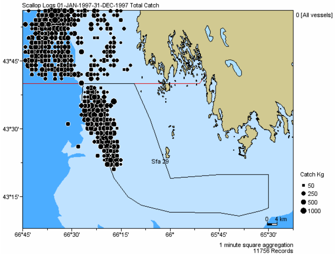
Fig. 5. Location of commercial catches from fishing logs of the Full Bay scallop fleet in 1997.
