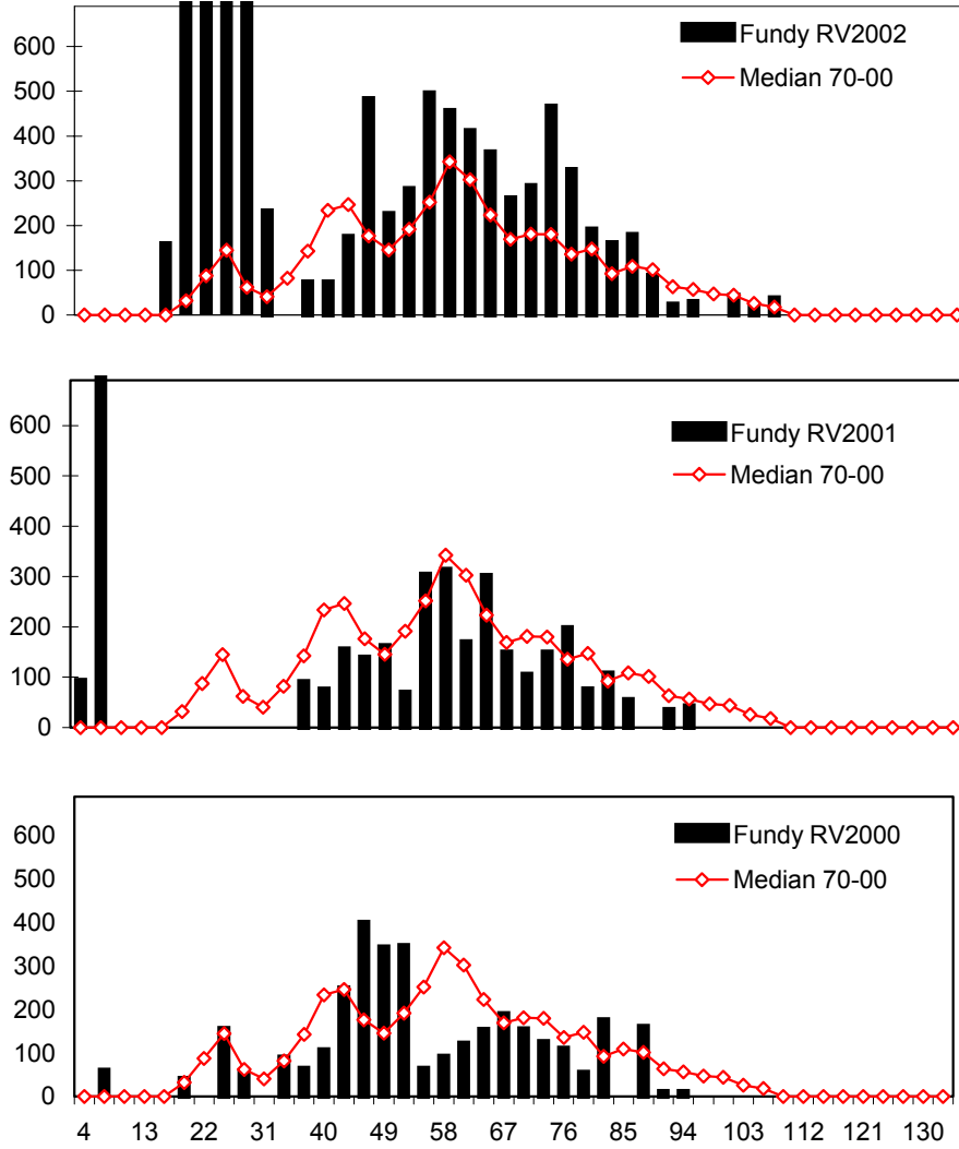
Fig. 19. Fundy length frequencies from summer RV surveys compared to the long-term median.
