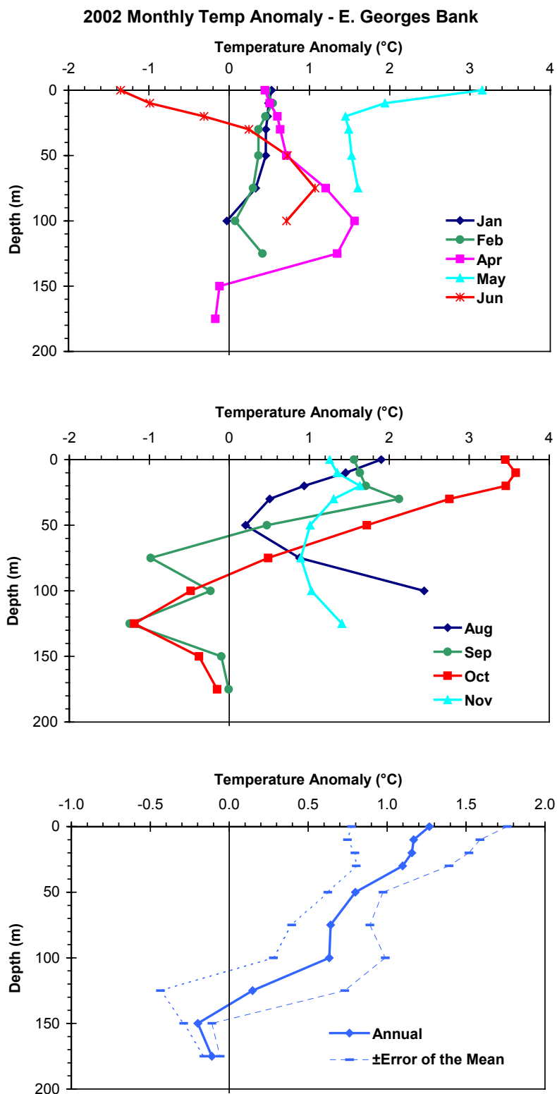
Fig. 16. The 2002 monthly temperature anomaly profiles (top two panels) and the annual anomalies with the standard error of the mean (bottom panel) for Eastern Georges Bank (area 28-Fig. 8).
