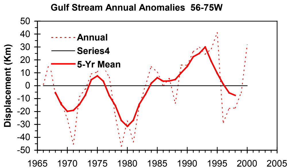
Fig.28. The 2002 (dashed line) and long-term mean (1973-2000; solid line) positions of the northern edge of the Gulf Stream (top panel) and the time series of the annual anomaly of the mean (56°-75°W) position of the Gulf Stream front (bottom panel).
