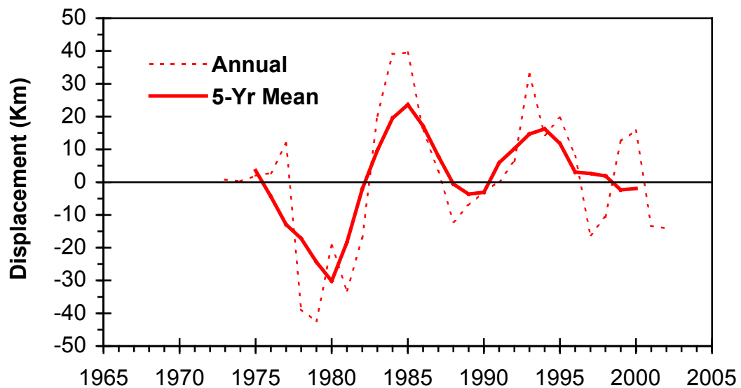
Fig.27. The 2002 (dashed line) and long-term mean (1973-2000; solid line) positions of the shelf/slope front (top panel) and the time series of the annual anomaly of the mean (56°-75°W) position of the shelf/slope front (bottom panel).
