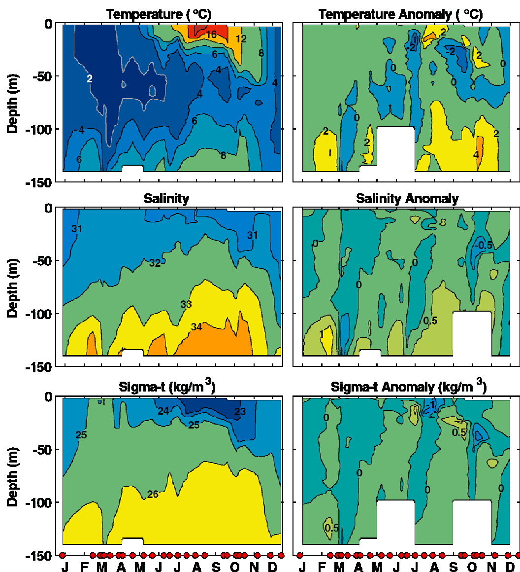
Fig. 6. Contours by depth of the 2002 temperature, salinity and density (sigma-t) (left) and their anomalies (right) at the standard station H2. The circles at the bottom of the figure indicate sampling dates.
