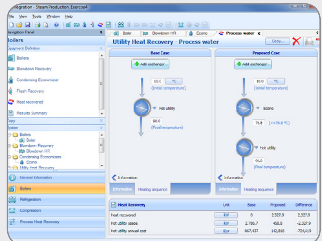
Heat recovery from utility system for both existing and improved situations, side-by-side
