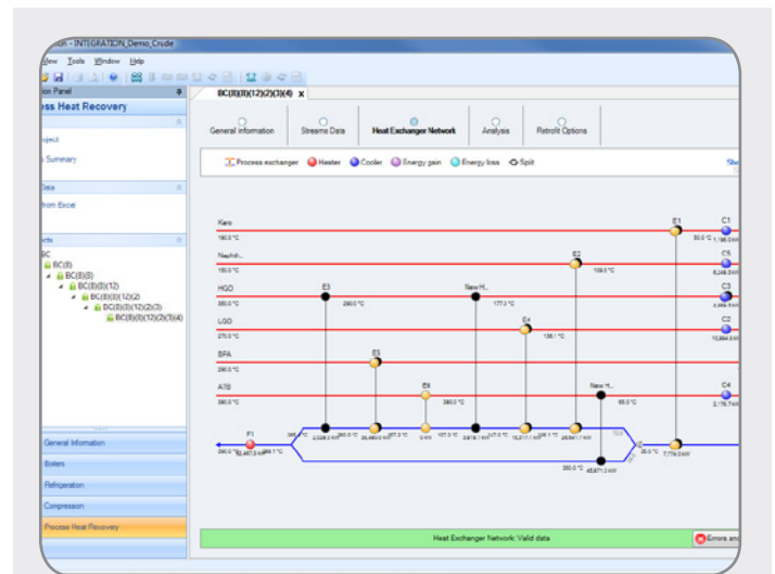
Optimized heat exchanger network after several changes to increase heat recovery
