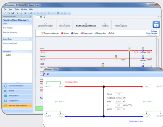
Heat exchanger network (grid diagram) and editor for individual exchanger
