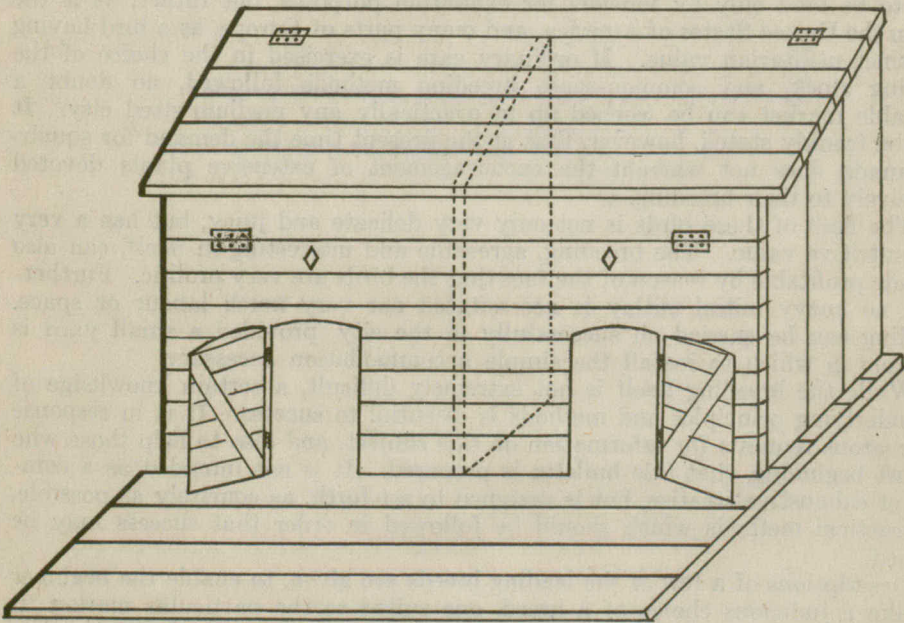
Fig. 1.—Hanging Pigeon Box
